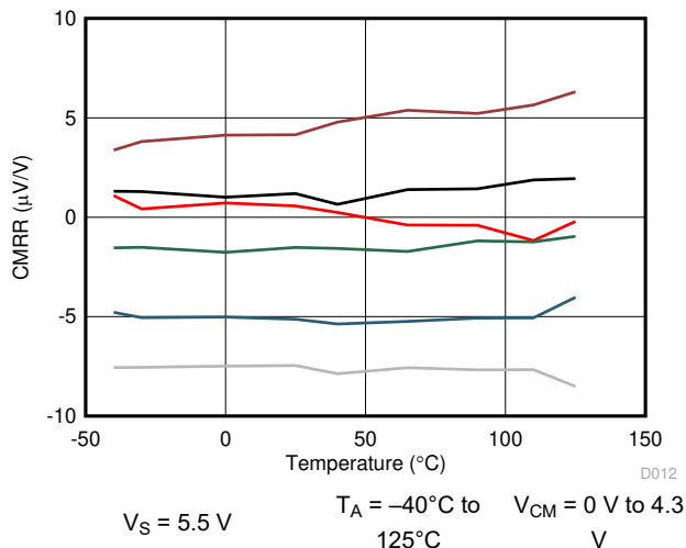
7-14. CMRR vs Temperature
