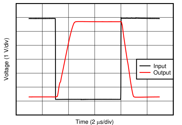
7-30. Overload Recovery
