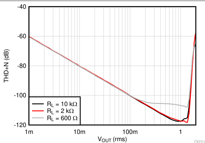
7-70. THD + N vs Amplitude
