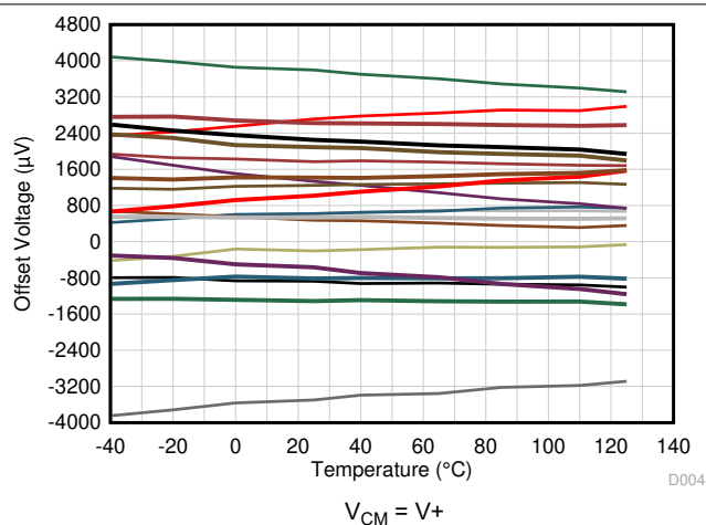
7-42. Offset Voltage vs Temperature (NMOS Input Pair)
