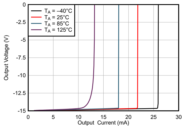
Figure 6-29. Output Voltage Swing vs Output Sinking Current
