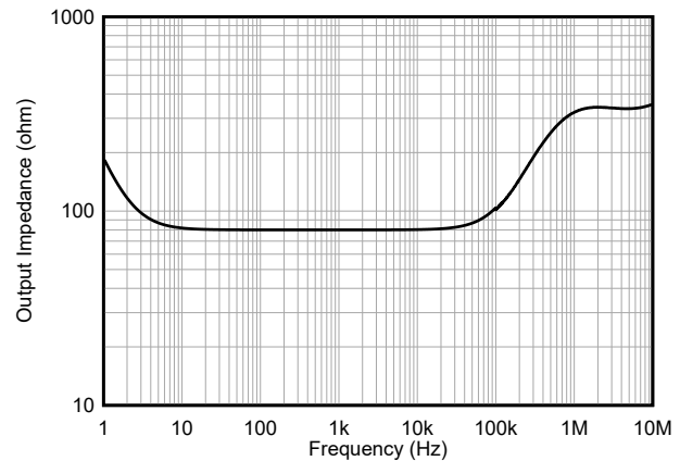
Figure 6-30. Open-Loop Output Impedance vs Frequency
