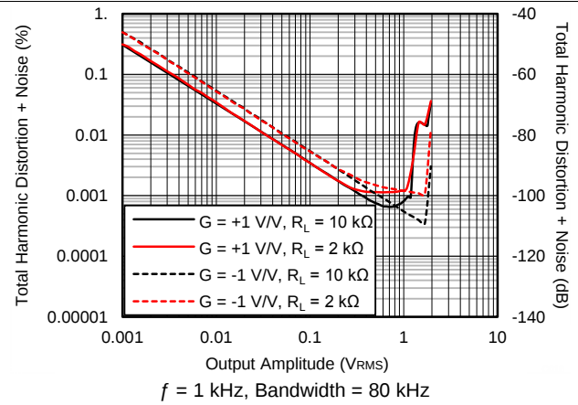
FIG 20. THD + N vs Amplitude
