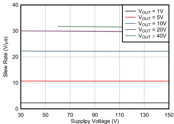
FIG 6-44. Slew Rate vs Supply Voltage (Inverting)
