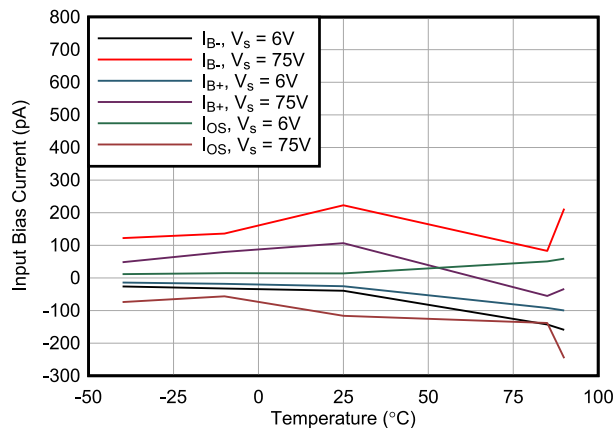
FIG 6-20. IB vs Temperature
