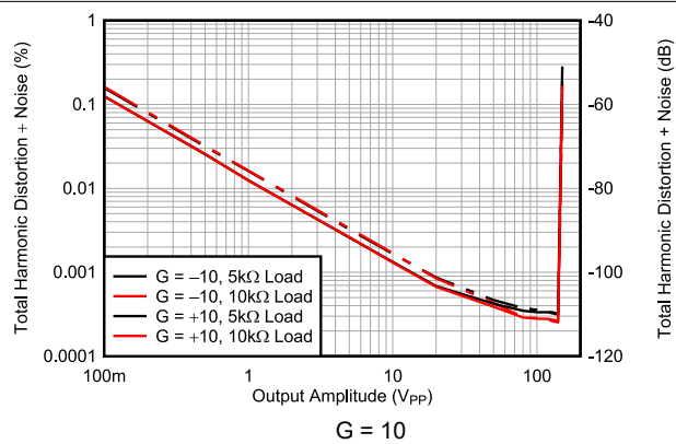
FIG 6-48. THD+N Ratio vs Output Amplitude
