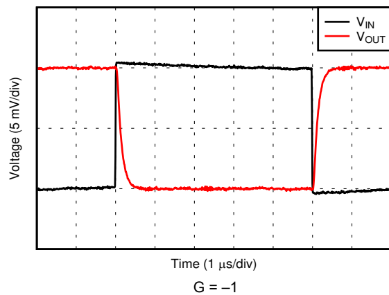
6-39. Small-Signal Step Response
