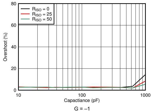
6-37. Small-Signal Overshoot vs Capacitive Load
