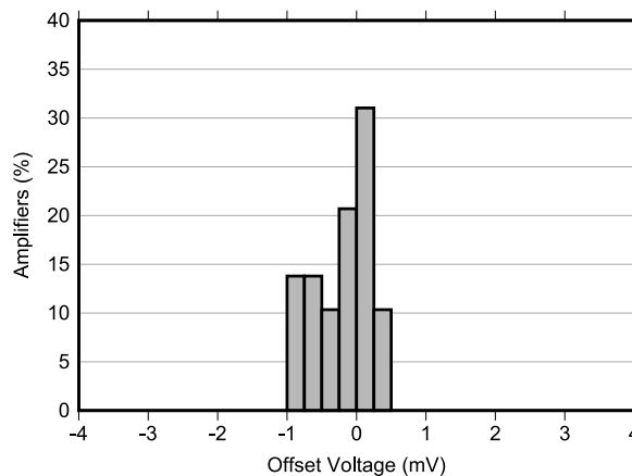
FIG 6-2. Offset Voltage Distribution at 85°C
