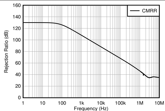
6-14. CMRR vs Frequency
