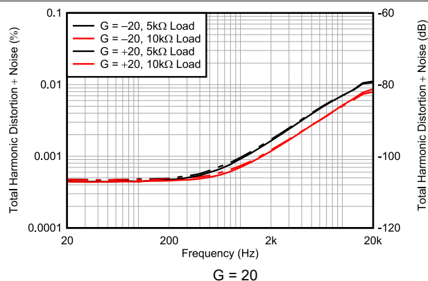
FIG 6-47. THD+N Ratio vs Frequency
