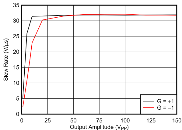
FIG 6-43. Slew Rate vs Output Step Size
