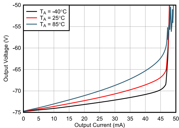
FIG 6-31. Negative Output Voltage vs Output Current
