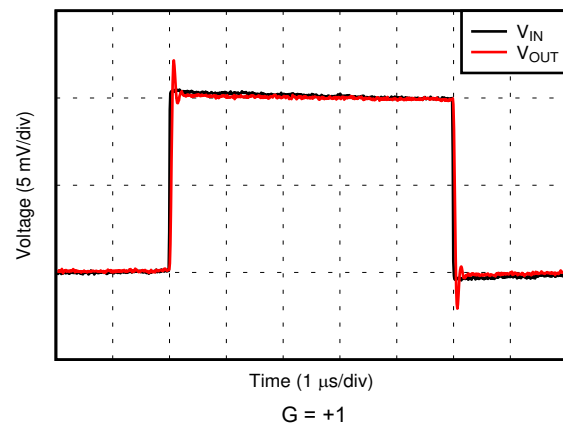
6-40. Small-Signal Step Response
