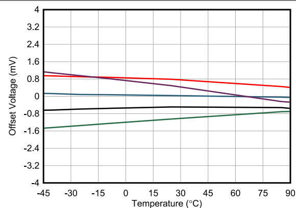
FIG 6-5. Offset Voltage vs Temperature
