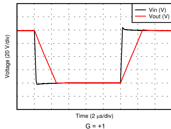
6-42. Large-Signal Step Response
