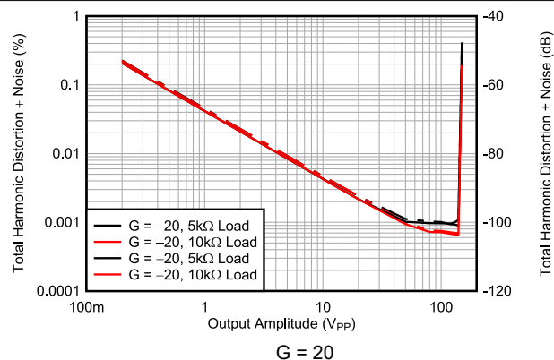
Figure 6-49. THD+N Ratio vs Output Amplitude
