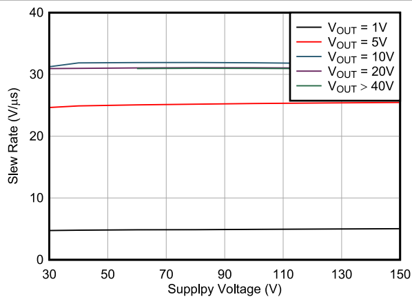
FIG 6-45. Slew Rate vs Supply Voltage (Noninverting)
