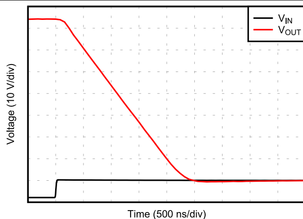
FIG 6-34. Positive Overload Recovery
