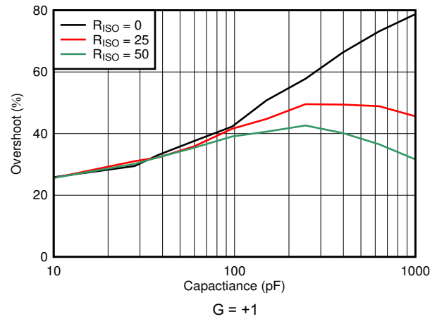
6-38. Small-Signal Overshoot vs Capacitive Load
