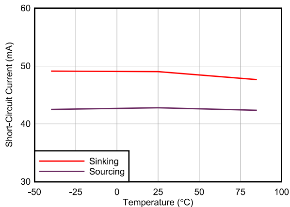
FIG 6-32. Short-Circuit Current vs Temperature
