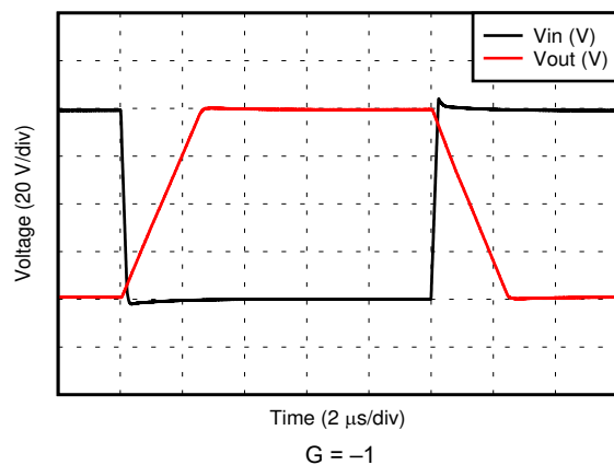
6-41. Large-Signal Step Response
