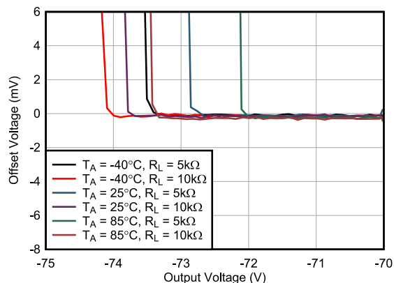
Figure 6-11. Offset Voltage vs Output Voltage (Low Output)
