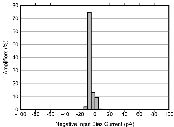
FIG 6-19. Input Bias Current Production Distribution at 25^\circ\text{C}
