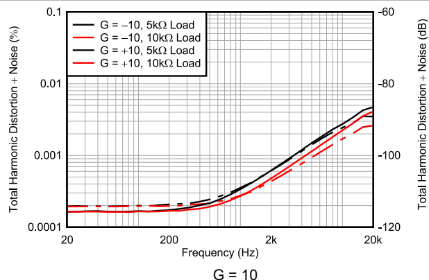
FIG 6-46. THD+N Ratio vs Frequency
