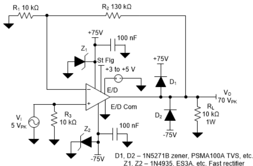
図 8-1. OPA455, High-Voltage Noninverting Amplifier, A_v = 14 V/V
