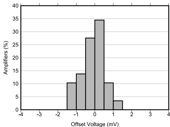
FIG 6-1. Offset Voltage Distribution at 25°C
