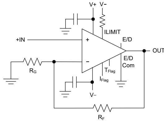
8-4. Schematic Representation
