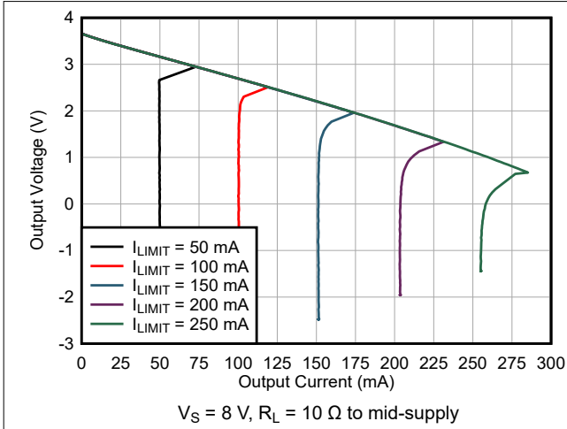
6-31. Output Voltage vs Current Limit Set
