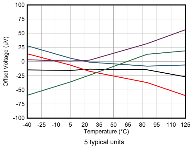
6-9. Input Offset Voltage vs Temperature
