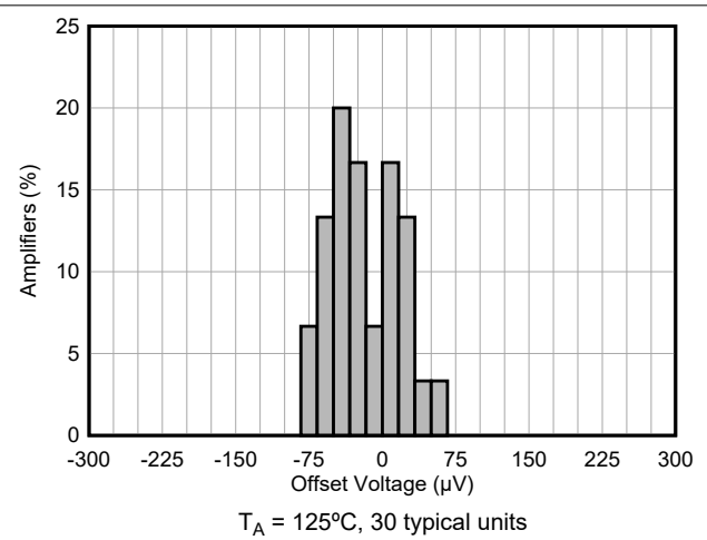
6-4. Input Offset Production Distribution
