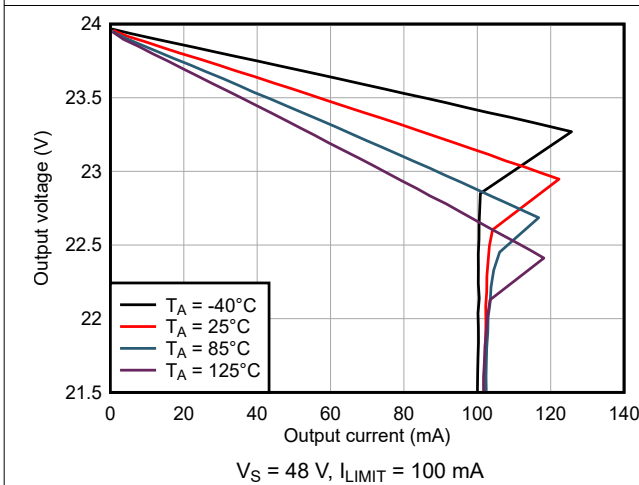
6-21. Output Voltage vs Output Sourcing Current
