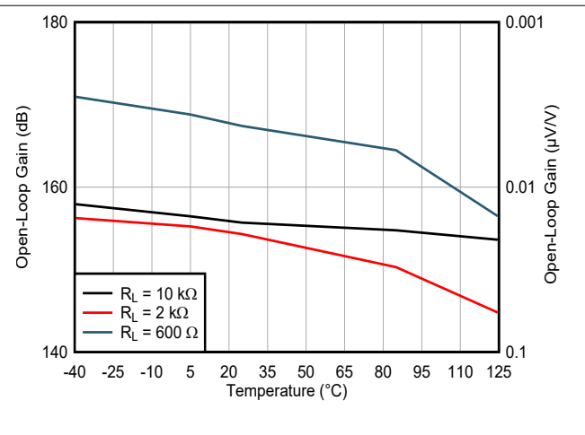
6-16. Open Loop Gain vs Temperature
