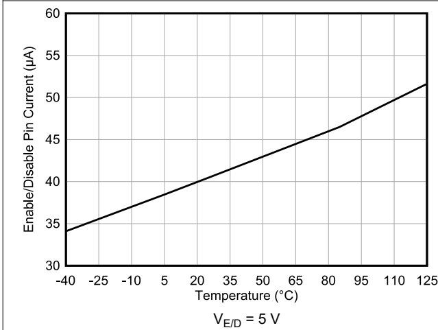
6-69. Enable/Disable Pin Current vs Temperature
