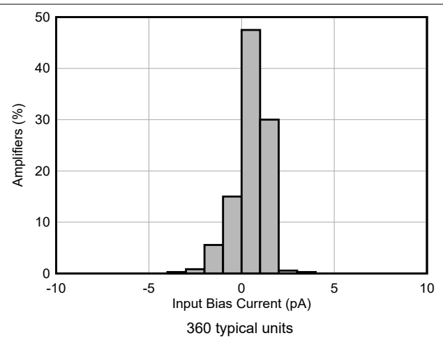
6-6. Input Bias Current Production Distribution
