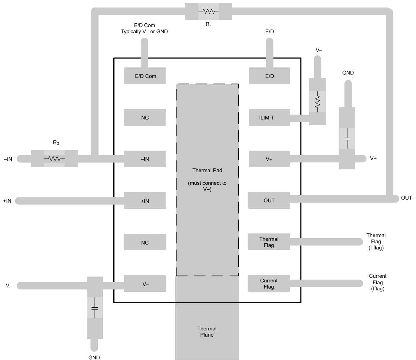
8-5. OPA593 Board Layout for Noninverting Configuration
