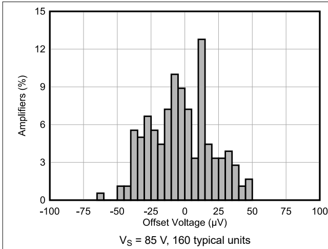
6-1. Input Offset Production Distribution
