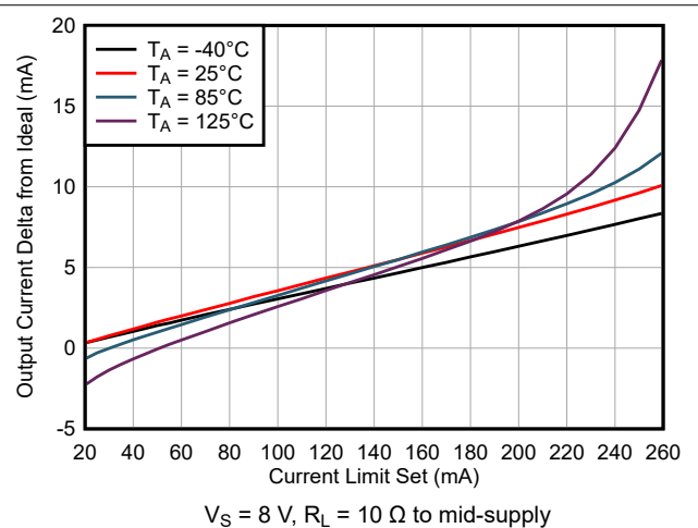
6-36. Output Sinking Current Error vs Current Limit Set
