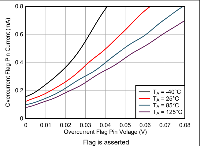
6-72. Current-Limit Flag Pin vs Current-Limit Flag Pin Voltage
