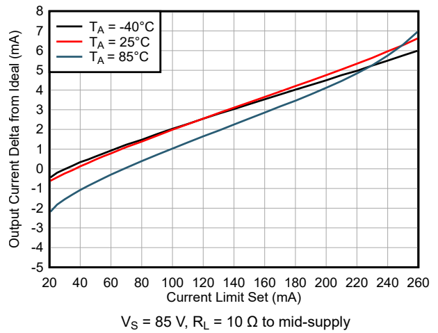
6-38. Output Sinking Current Error vs Current Limit Set
