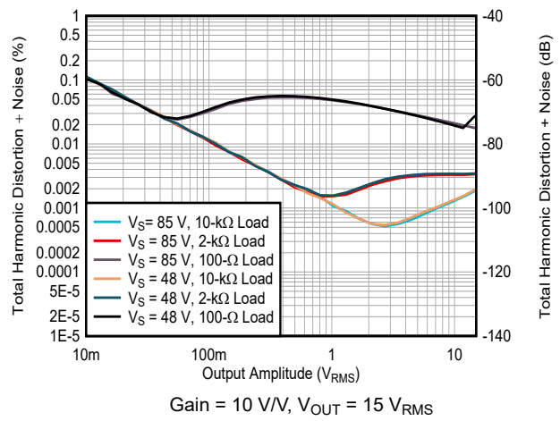
6-48. Total Harmonic Distortion + Noise vs Amplitude
