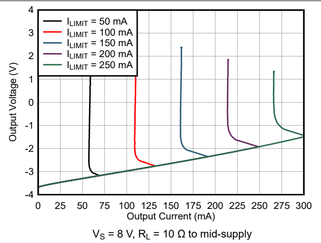
6-32. Output Voltage vs Current Limit Set
