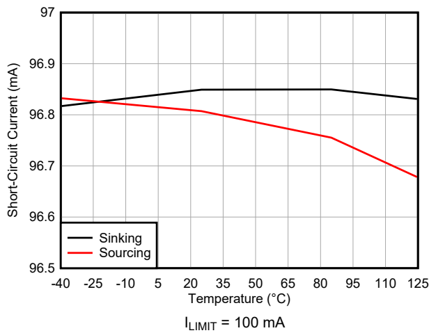
6-39. Short Circuit Current vs Temperature
