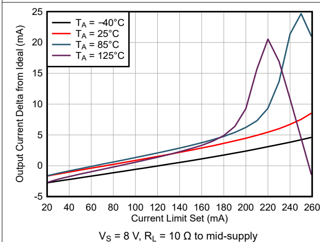
6-35. Output Sourcing Current Error vs Current Limit Set
