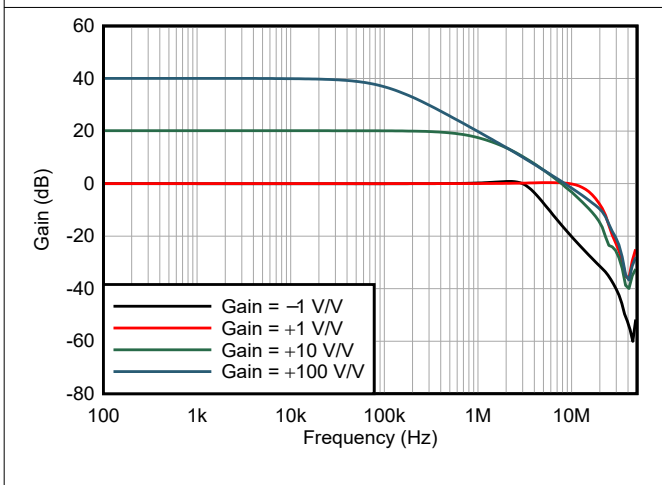
6-17. Closed-Loop Gain vs Frequency
