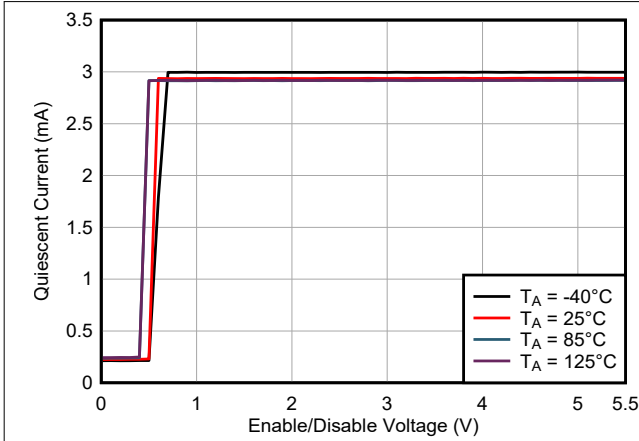
6-67. Quiescent Current vs Enable Voltage
