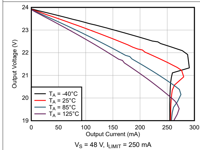
Fig 6-27. Output Voltage vs Output Sourcing Current
