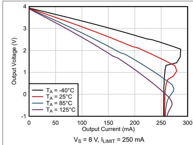
Fig 6-25. Output Voltage vs Output Sourcing Current
