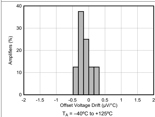
6-5. Input Offset Voltage Drift Distribution
