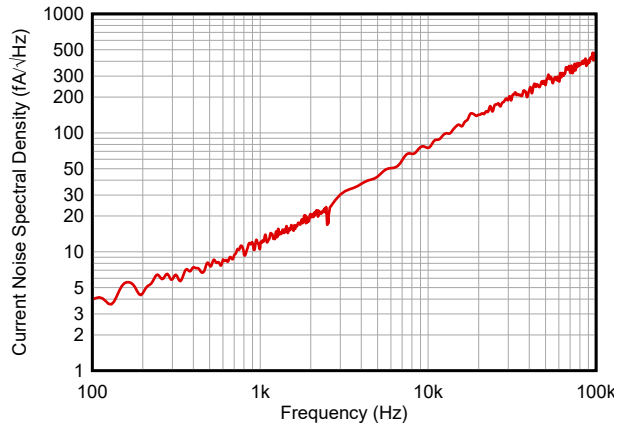
6-44. Input Current Noise Spectral Density
