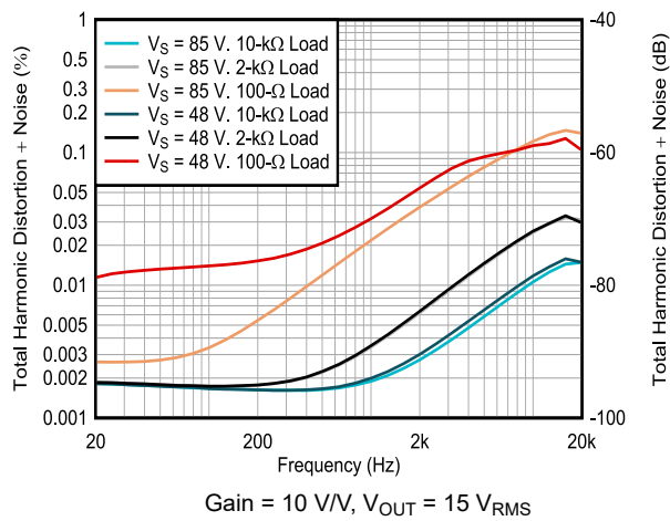
6-47. Total Harmonic Distortion + Noise vs Frequency
