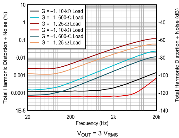
6-45. Total Harmonic Distortion + Noise vs Frequency
