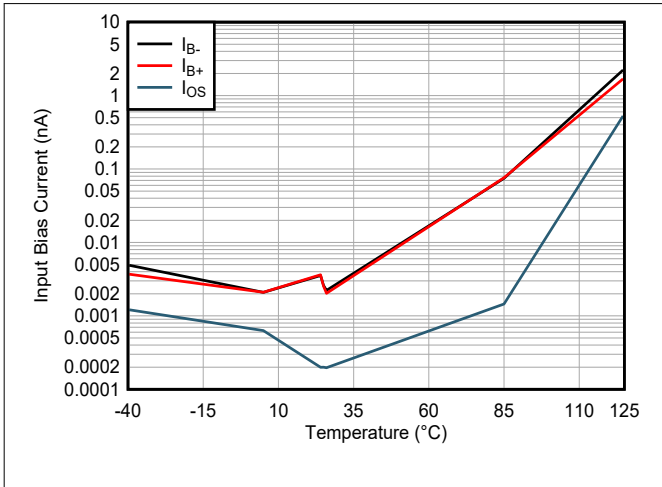
6-13. Input Bias Current and Current Offset vs Temperature
