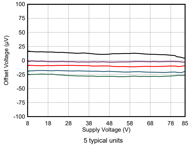
6-8. Input Offset Voltage vs Supply Voltage
