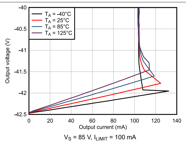
6-24. Output Voltage vs Output Sinking Current
