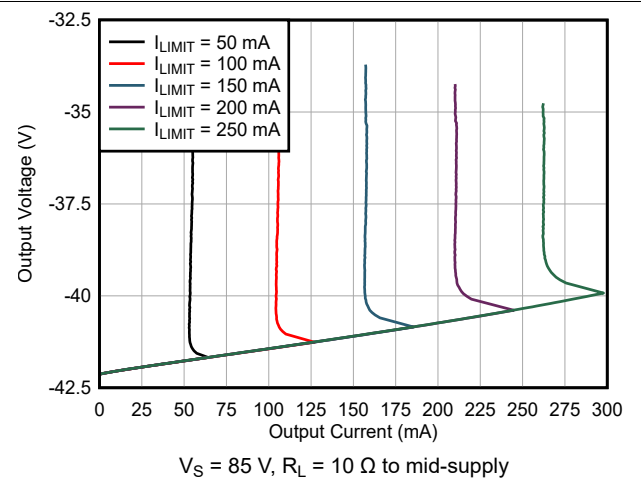
6-34. Output Voltage vs Output Sinking Current
