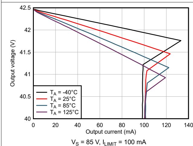
6-23. Output Voltage vs Output Sourcing Current
