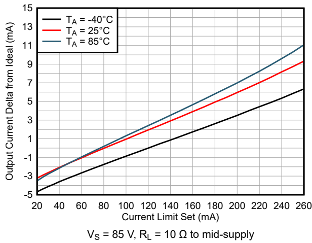
6-37. Output Sourcing Current Error vs Current Limit Set
