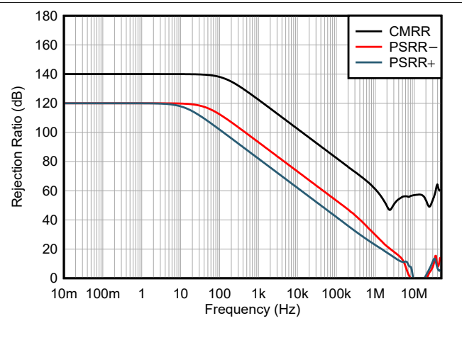
6-14. PSRR and CMRR vs Frequency
