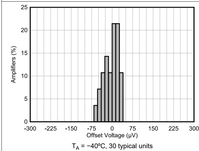
6-3. Input Offset Production Distribution
