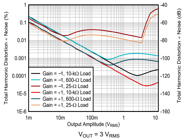
6-46. Total Harmonic Distortion + Noise vs Amplitude
