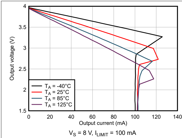
6-19. Output Voltage vs Output Sourcing Current
