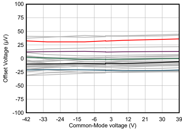
6-7. Input Offset Voltage vs Common-Mode Voltage
