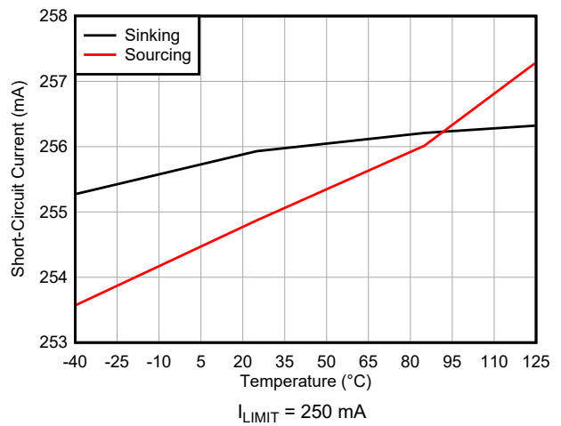
6-40. Short Circuit Current vs Temperature
