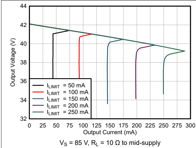
6-33. Output Voltage vs Output Sourcing Current
