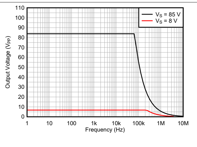
6-18. Maximum Output Voltage vs Frequency
