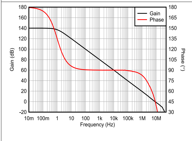
6-15. Open-Loop Gain and Phase vs Frequency
