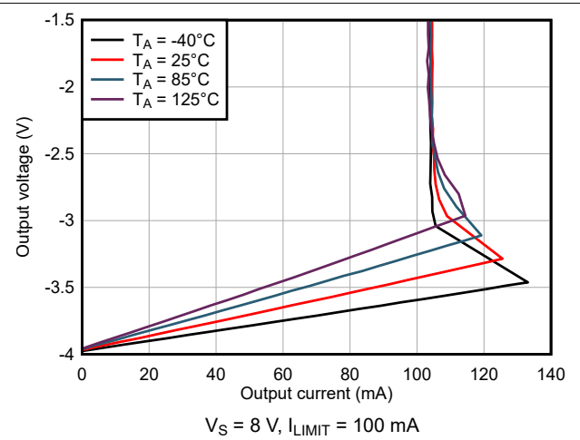
6-20. Output Voltage vs Output Sinking Current
