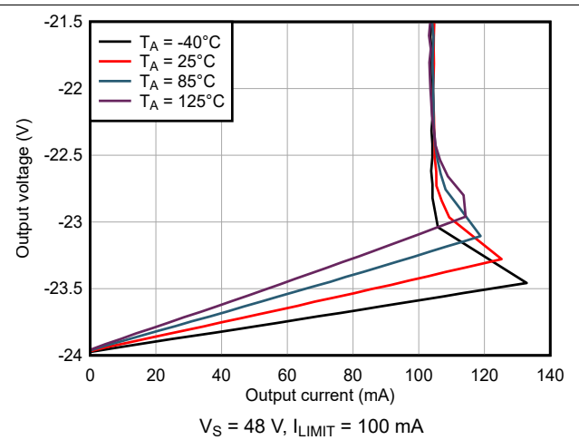
6-22. Output Voltage vs Output Sinking Current
