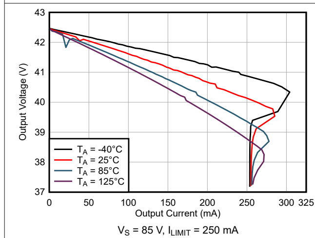
Fig 6-29. Output Voltage vs Output Sourcing Current
