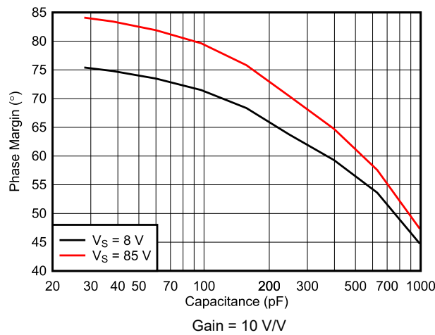
Figure 6-51. Phase Margin vs Capacitive Load
