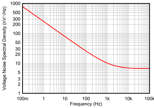
6-43. Input Voltage Noise Spectral Density
