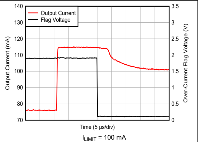
6-68. Current Limit Response
