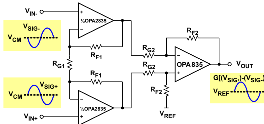
FIG 9-1. Instrumentation Amplifier
