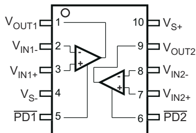
FIG 6-3. OPA2835: DGS Package 10-Pin VSSOP Top View
