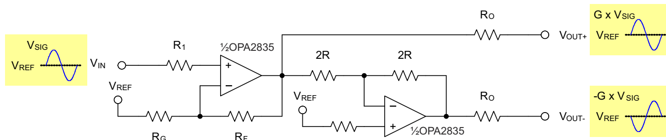
FIG 9-2. Single-Ended to Differential Amplifier
