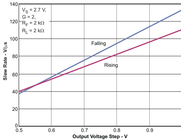
7-5. Slew Rate vs Output Voltage Step
