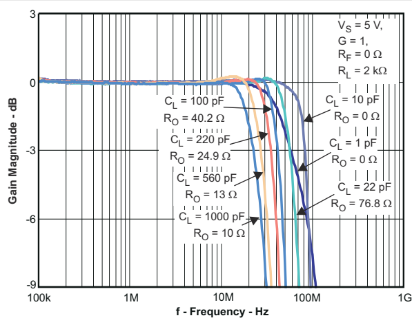
7-40. Frequency Response With Capacitive Load
