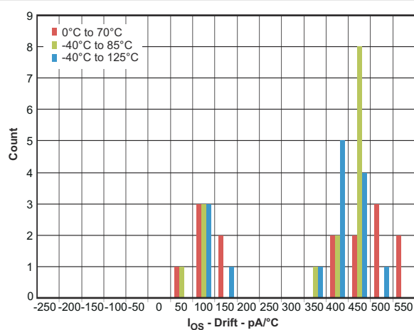
FIG 7-52. Input Offset Current Drift
