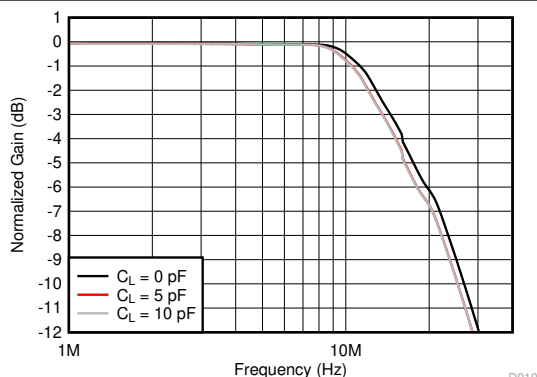
Figure 6-20. Large-Signal Frequency Response
