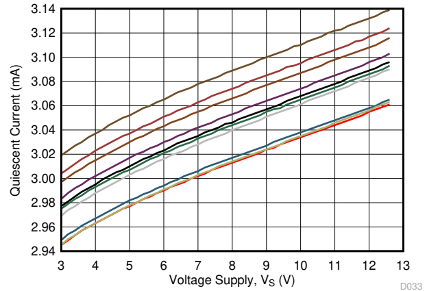
Figure 6-48. Quiescent Current vs Voltage Supply
