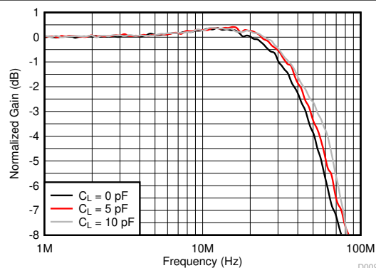
Figure 6-19. Small-Signal Frequency Response
