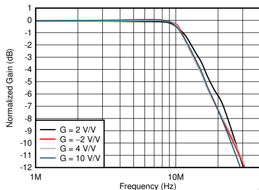
Figure 6-20. Large-Signal Frequency Response
