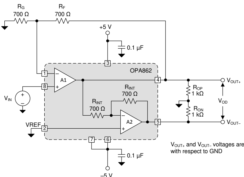
8-1. Single-Ended To Differential Gain of 4 V/V Configuration
