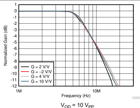
Figure 6-2. Large-Signal Frequency Response
