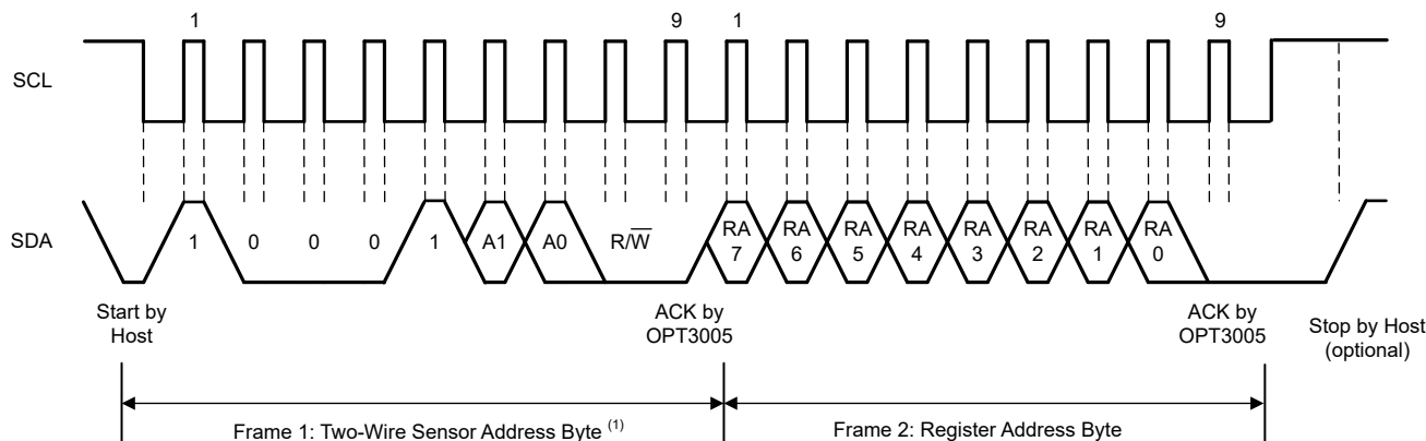
Figure 8-1. Setting the I 2 C Register Address
