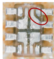
FIG 9-8. Identifying Package Orientation - Backside
