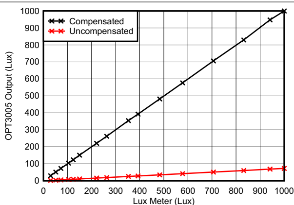
図 9-5. Uncompensated and Compensated Output of the OPT3005 Under a Dark Window Illuminated by Fluorescent Light Source
