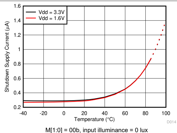
Figure 7-11. Shutdown Current vs Temperature
