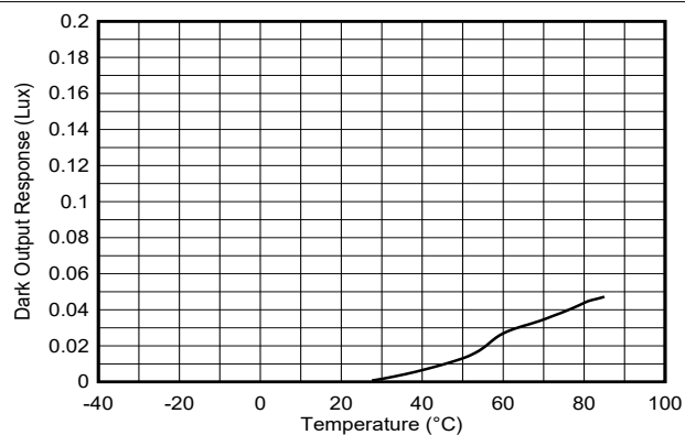
7-3. Dark Response vs Temperature
