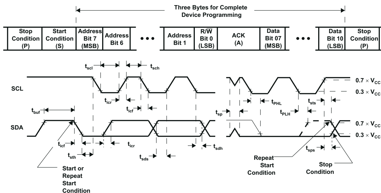
VOLTAGE WAVEFORMS
