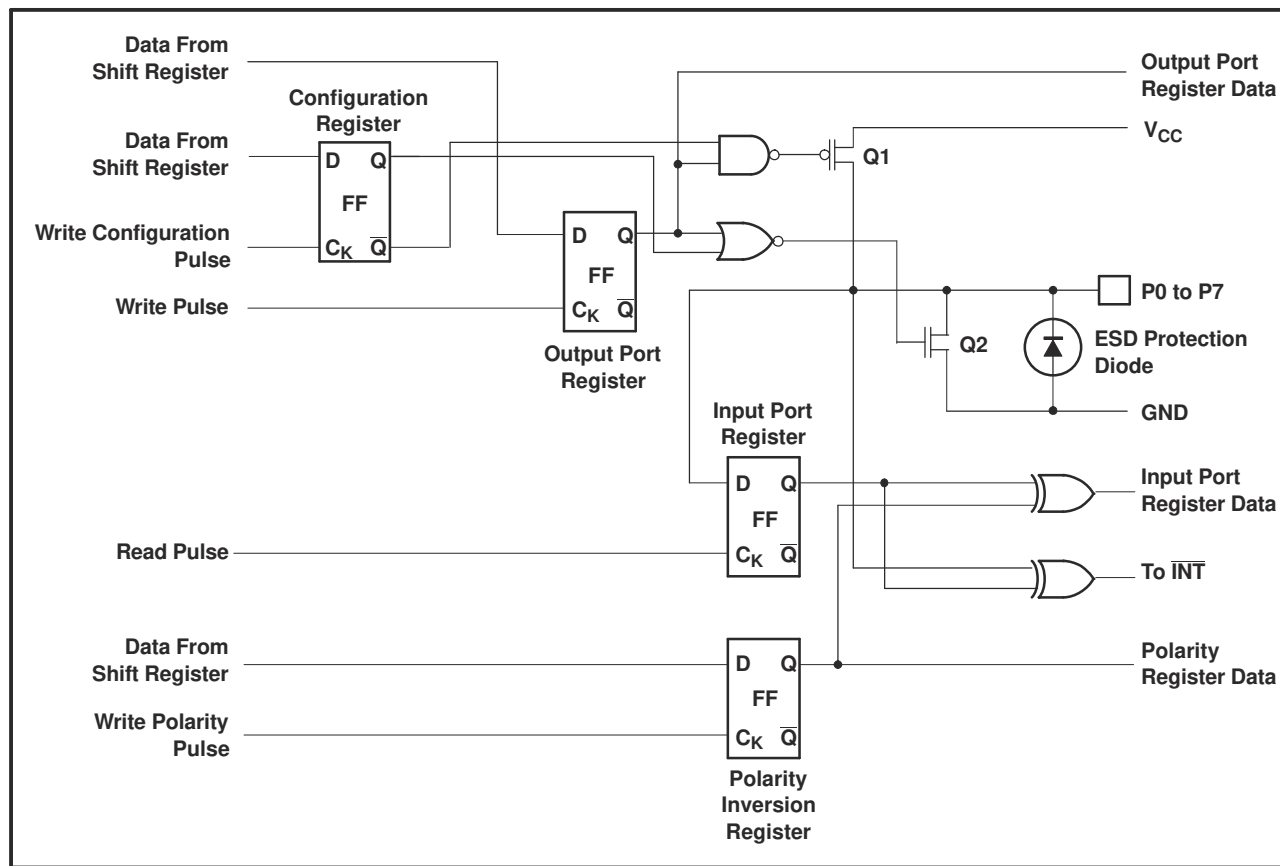
9-2. Simplified Schematic of P0 to P7
