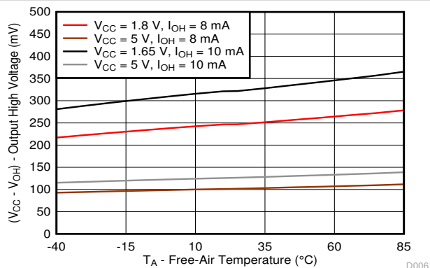
5-6. Output High Voltage ( V_{CC} - V_{OH} ) vs Temperature ( T_A ) for P-Ports
