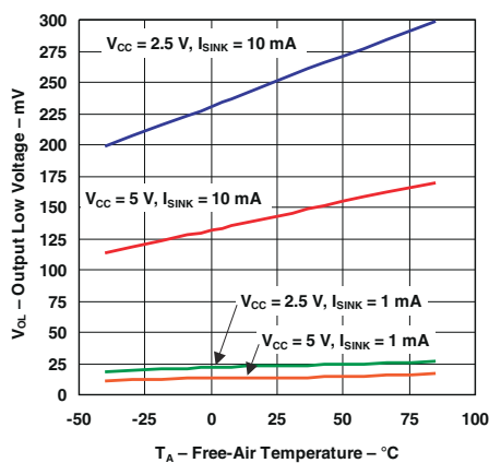
図 5-12. Output Low Voltage vs Temperature
