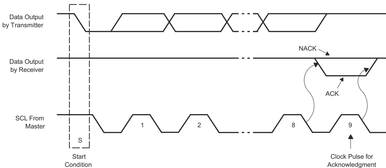
図 7-6. Acknowledgment on the I 2 C Bus
