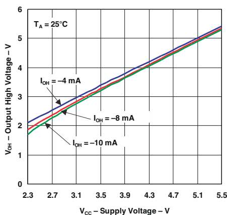
図 5-10. Output High Voltage vs Supply Voltage (P7-P1)
