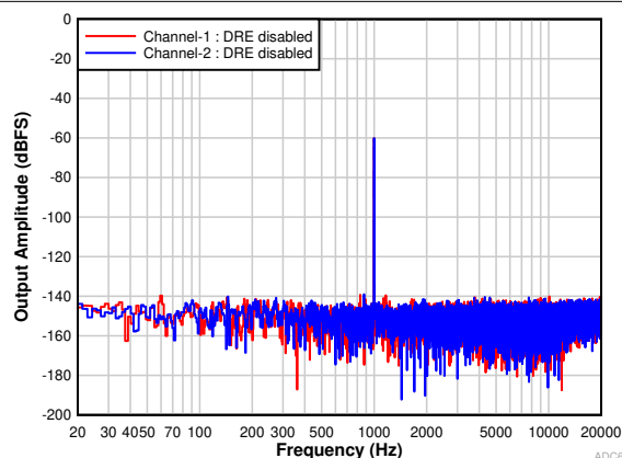
9-4. PCM1820: FFT With a –60-dBr Input With DRE Disabled
