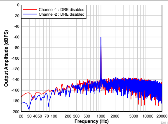
7-9. PCM1820: FFT With Idle Input and DRE Disabled
