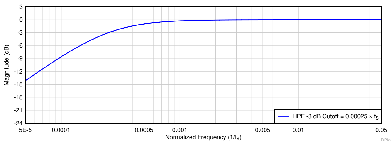
图 8-6. HPF Filter Frequency Response Plot
