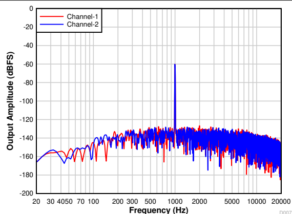
7-19. PCM1821: FFT With a -60-dBr Input
