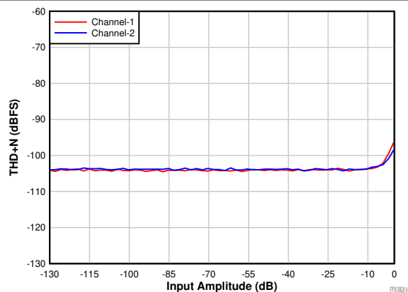
9-7. PCM1821: THD+N vs Input Amplitude
