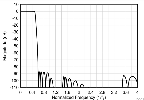
Figure 8-21. Low-Latency Decimation Filter Magnitude Response
