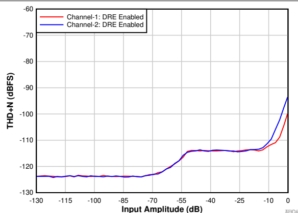
9-3. PCM1820: THD+N vs Input Amplitude With DRE Enabled
