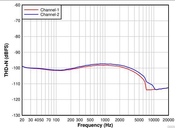
7-3. PCM1820: THD+N vs Input Frequency With a -60-dBr Input
