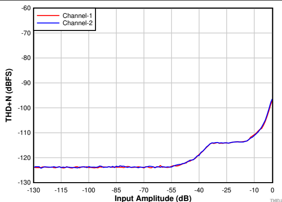
7-1. PCM1820: THD+N vs Input Amplitude With DRE Enabled
