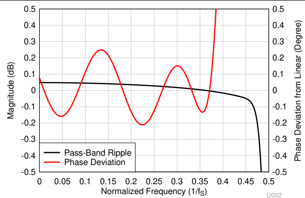
Figure 8-22. Low-Latency Decimation Filter Pass-Band Ripple and Phase Deviation
