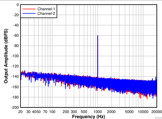
9-6. PCM1821: FFT With a –60-dBr Input
