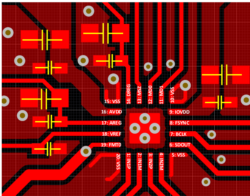
11-1. Example Layout
