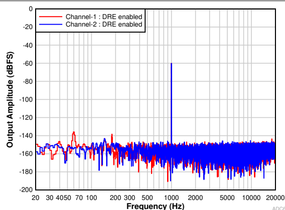
9-2. PCM1820: FFT With a –60-dBr Input With DRE Enabled
