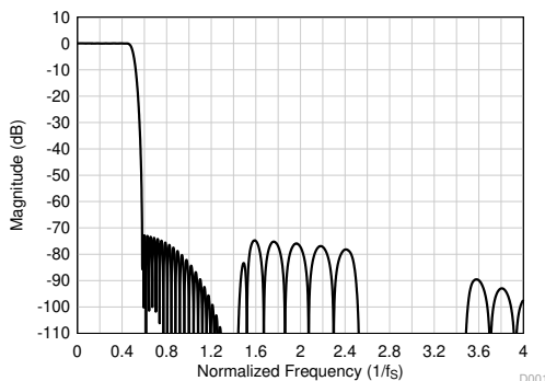
図 8-7. Linear Phase Decimation Filter Magnitude Response
