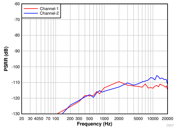
7-7. PCM1820: Power-Supply Rejection Ratio vs Ripple Frequency With a 100-mV PP Amplitude
