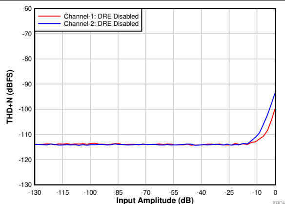
9-5. PCM1820: THD+N vs Input Amplitude With DRE Disabled
