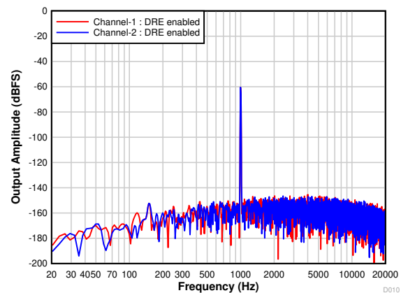
7-10. PCM1820: FFT With a -60-dBr Input and DRE Enabled
