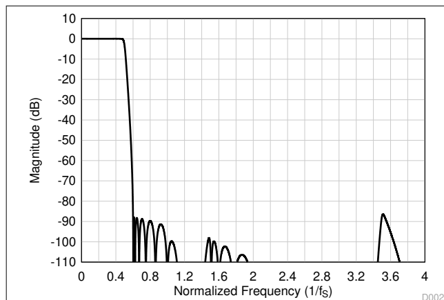
图 8-27. Low-Latency Decimation Filter Magnitude Response
