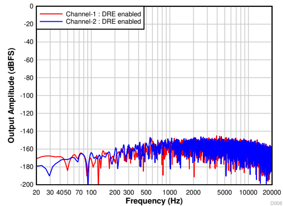
7-8. PCM1820: FFT With Idle Input and DRE Enabled
