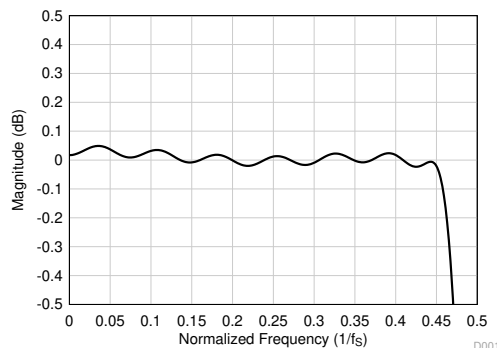
図 8-8. Linear Phase Decimation Filter Pass-Band Ripple
