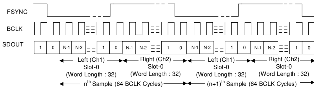
Figure 8-4. I 2 S Protocol Timing (FMT0 = LOW) In Master Mode
