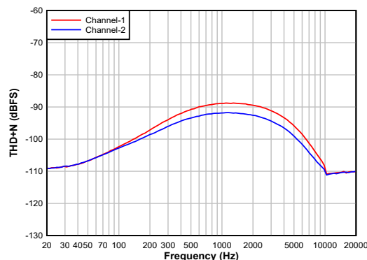
FIG 7-16. Single-Ended Input: THD+N vs Input Frequency With a -1-dBr Input
