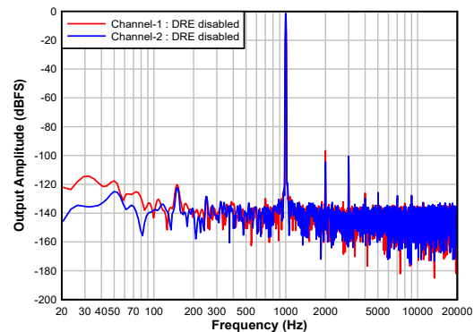
FIG 7-12. Differential Input: FFT With a -1-dBr Input
