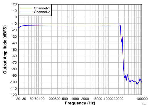
FIG 7-17. Single-ended Input: Frequency Response With a -12-dBr Input
