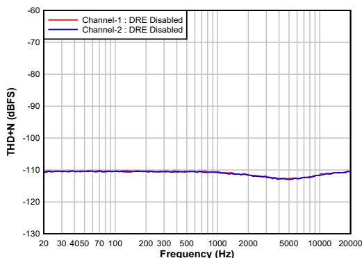
FIG 7-15. Single-Ended Input: DR vs Input Frequency With DRE Disabled
