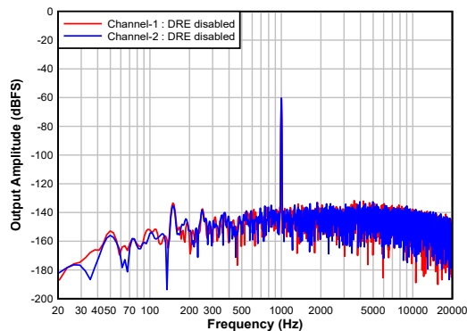
FIG 7-11. Differential Input: FFT With a -60-dBr Input and DRE Disabled
