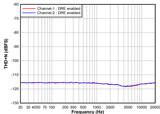
FIG 7-14. Single-ended Input: DR vs Input Frequency With DRE Enabled
