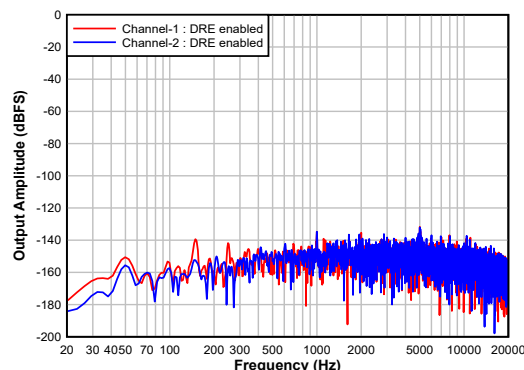
FIG 7-18. Single-ended Input: FFT With Idle Input and DRE Enabled
