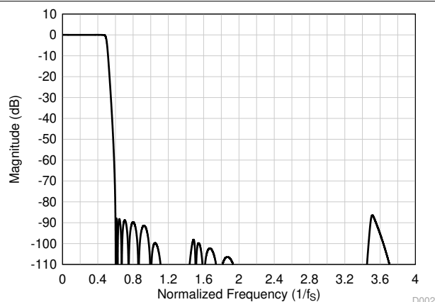
图 8-29. Low-Latency Decimation Filter Magnitude Response
