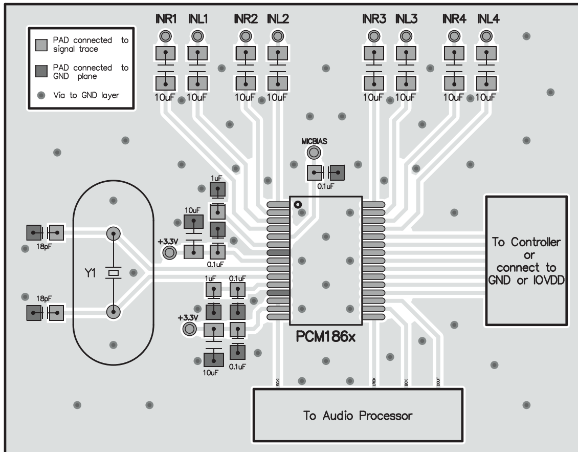
FIG 75. Layout Example
