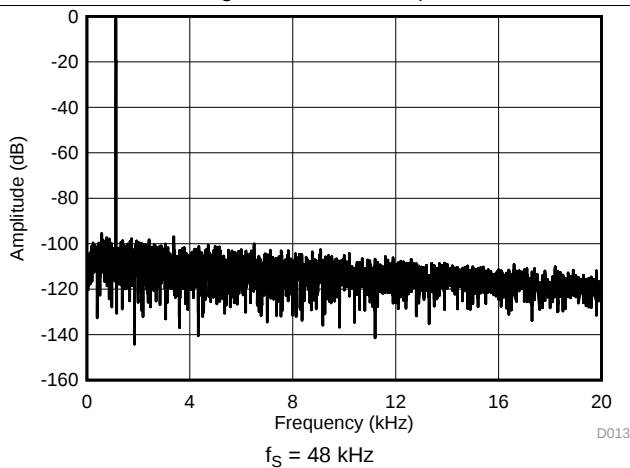
Figure 18. Secondary ADC FFT
