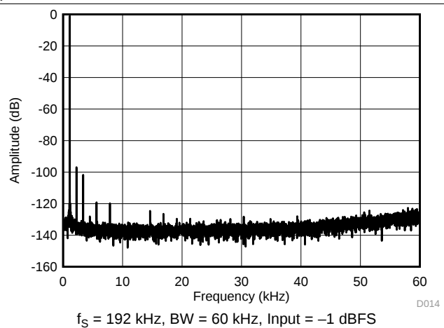
Figure 19. High Bandwidth FFT of THD Components
