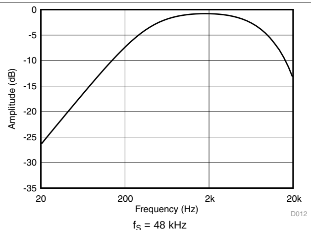
Figure 17. Secondary ADC Frequency Response
