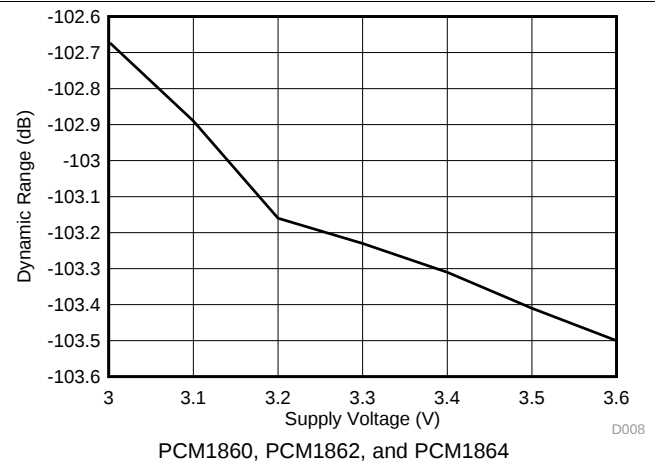
Figure 13. Dynamic Range vs Supply Voltage
