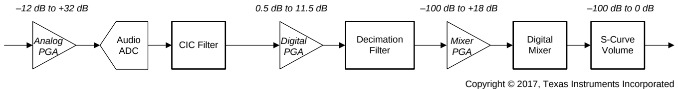
Figure 28. PCM186x Complete Gain Structure (PGAs and Attenuator)
