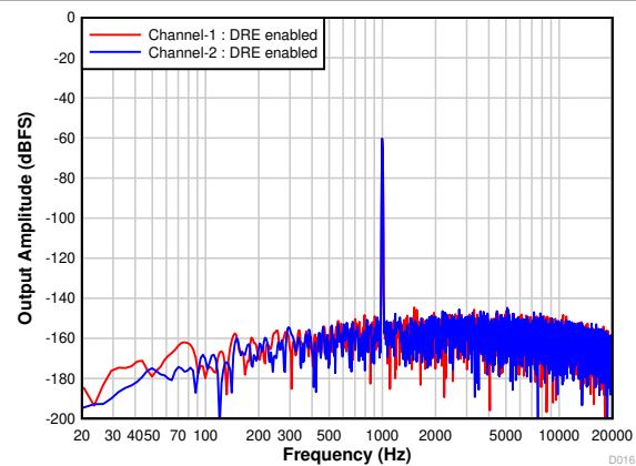
FIG 7-19. Differential FFT With a -60-dBr Input With DRE Enabled
