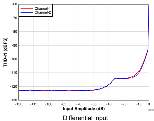
FIG 7-4. THD+N vs Input Amplitude With DRE Enabled
