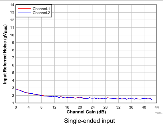
7-14. Input-Referred Noise vs Channel Gain
