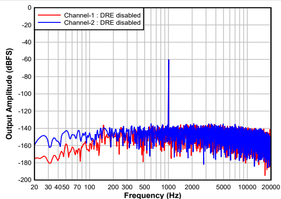
FIG 7-24. Single Ended FFT With a -60-dBr Input With DRE Disabled
