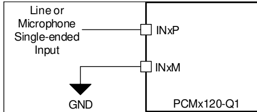
图 8-14. Single-Ended, DC-Coupled Input Connection
