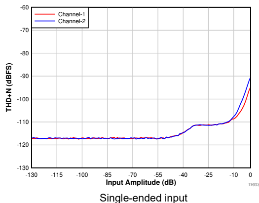
FIG 7-6. THD+N vs Input Amplitude With DRE Enabled
