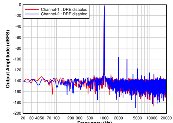
FIG 7-25. Differential FFT With a -1-dBr Input With DRE Disabled
