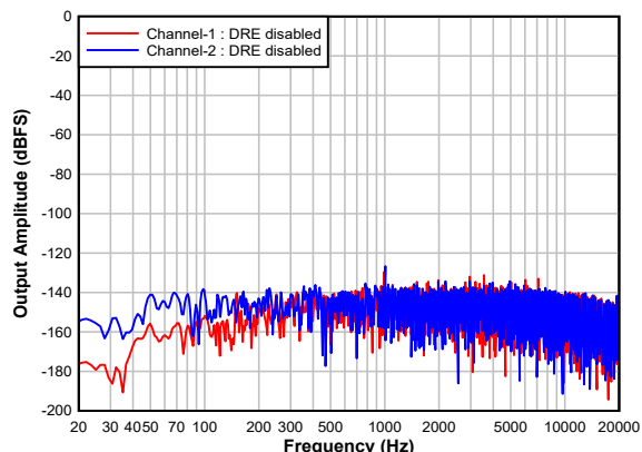
FIG 7-22. Single Ended FFT With Idle Input With DRE Disabled
