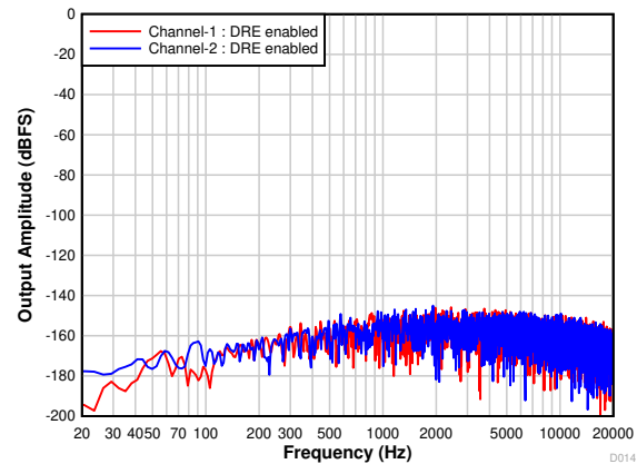
FIG 7-17. Differential FFT With Idle Input With DRE Enabled
