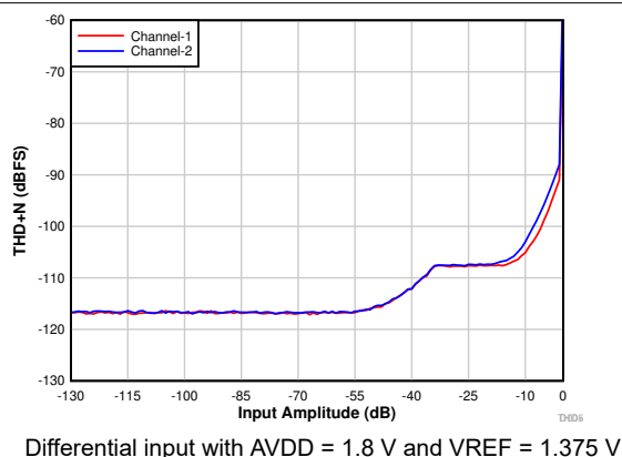
FIG 7-8. THD+N vs Input Amplitude With DRE Enabled
