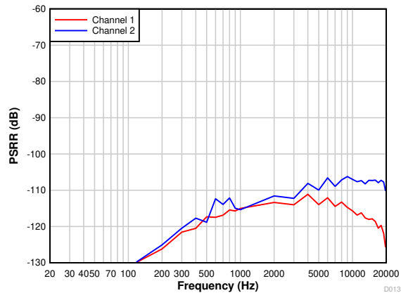
FIG 7-16. Power-Supply Rejection Ratio vs Ripple Frequency With 100-mV PP Amplitude
