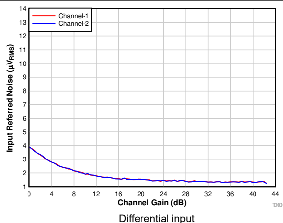
7-13. Input-Referred Noise vs Channel Gain
