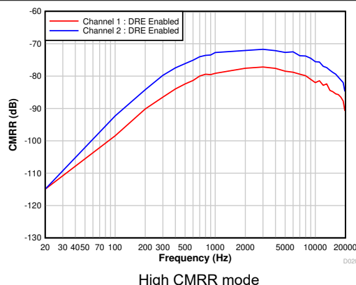
FIG 7-27. Common-Mode Rejection Ratio vs Ripple Frequency With 100-mV pp Amplitude and DRE Enabled
