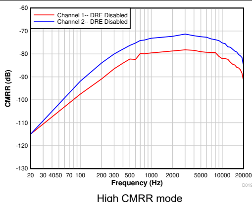
FIG 7-26. Common-Mode Rejection Ratio vs Ripple Frequency With 100-mV pp Amplitude and DRE Disabled
