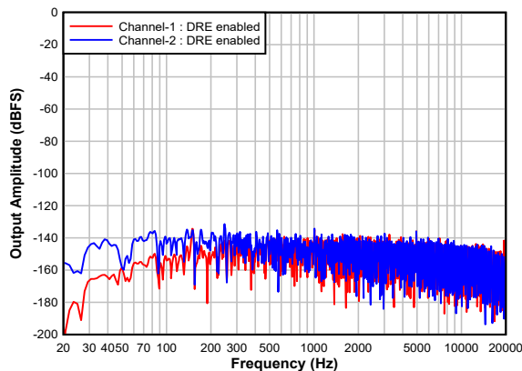
FIG 7-21. Single Ended FFT With Idle Input With DRE Enabled
