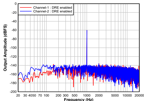
FIG 7-23. Single Ended FFT With a -60-dBr Input With DRE Enabled
