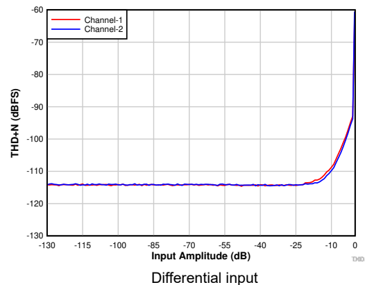
FIG 7-5. THD+N vs Input Amplitude With DRE Disabled
