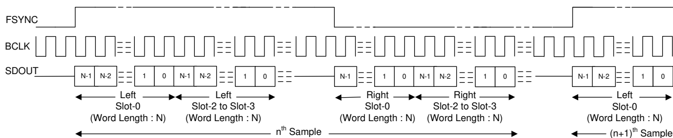
FIG 8-9. LJ Mode Standard Protocol Timing (TX_OFFSET = 0)
