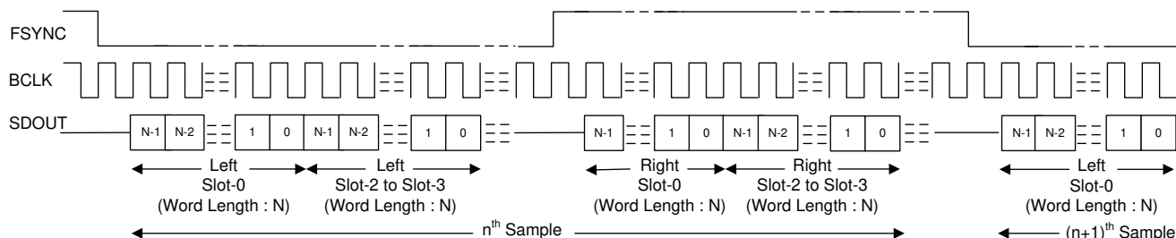
FIG 8-8. I²S Protocol Timing (TX_OFFSET = 0 and BCLK_POL = 1)
