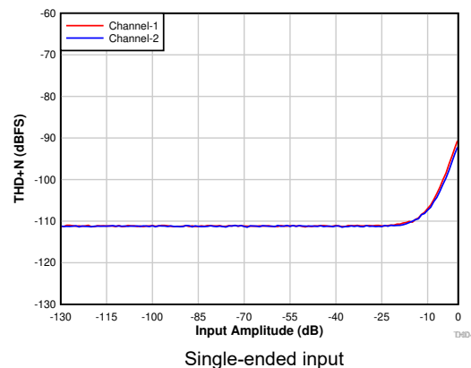
FIG 7-7. THD+N vs Input Amplitude With DRE Disabled
