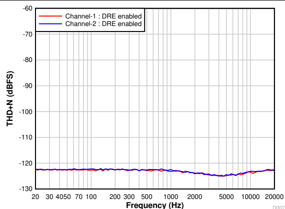
7-10. THD+N vs Input Frequency at -60\text{-dBr} Input With DRE Enabled
