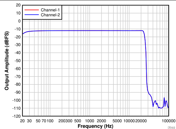
7-15. Frequency Response With a -12\text{-dBr} Input
