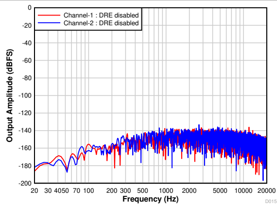
FIG 7-18. Differential FFT With Idle Input With DRE Disabled
