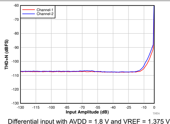
FIG 7-9. THD+N vs Input Amplitude With DRE Disabled
