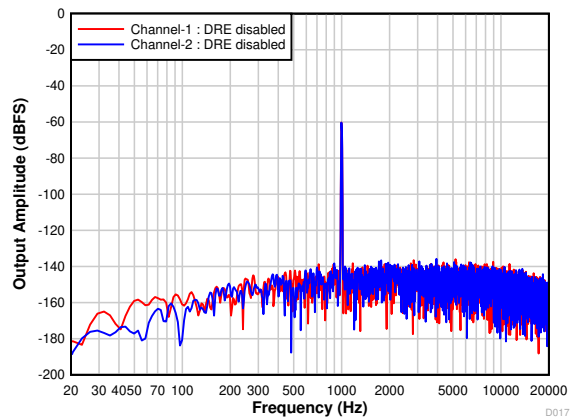
FIG 7-20. Differential FFT With a -60-dBr Input With DRE Disabled
