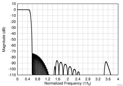
图 7-29. Linear Phase Decimation Filter Magnitude Response
