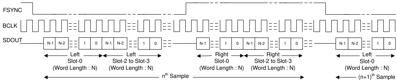
FIG 7-5. I 2 S Mode Standard Protocol Timing (TX_OFFSET = 0)
