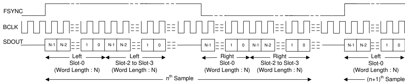
FIG 7-9. LJ Mode Standard Protocol Timing (TX_OFFSET = 0)
