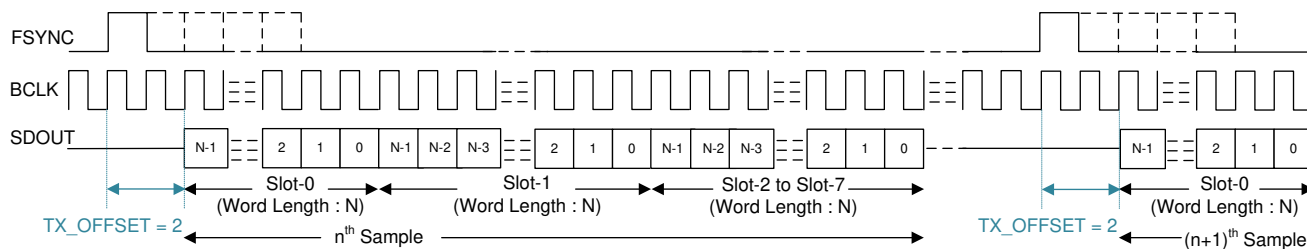
図 7-2. TDM Mode Protocol Timing (TX_OFFSET = 2)
