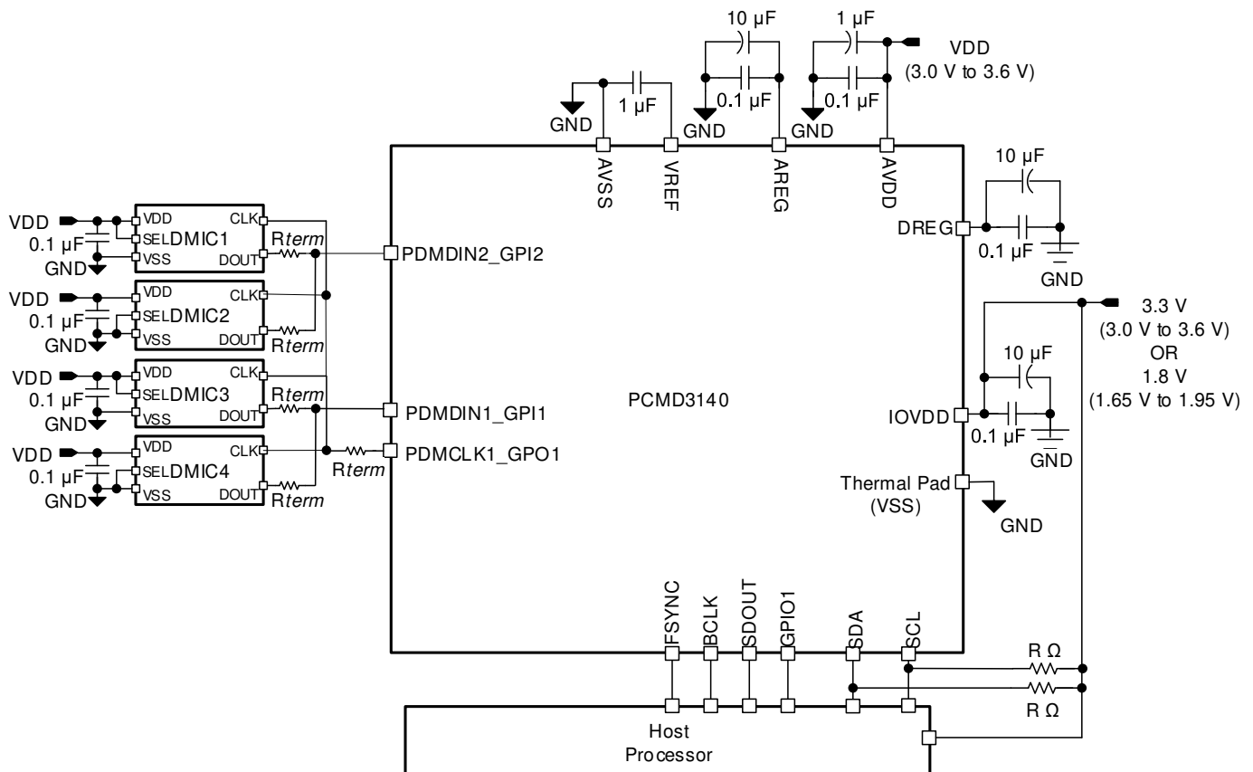
8-1. Four-Channel Digital PDM Microphone Recording Diagram
