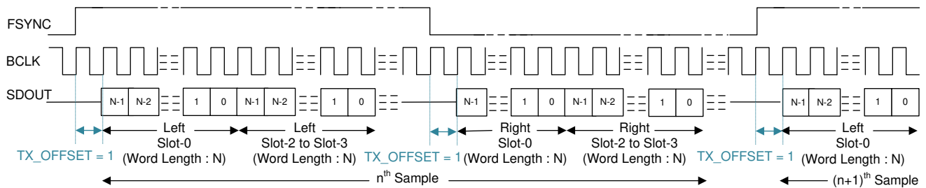
7-12. LJ Protocol Timing (TX_OFFSET = 1 and BCLK_POL = 1)
