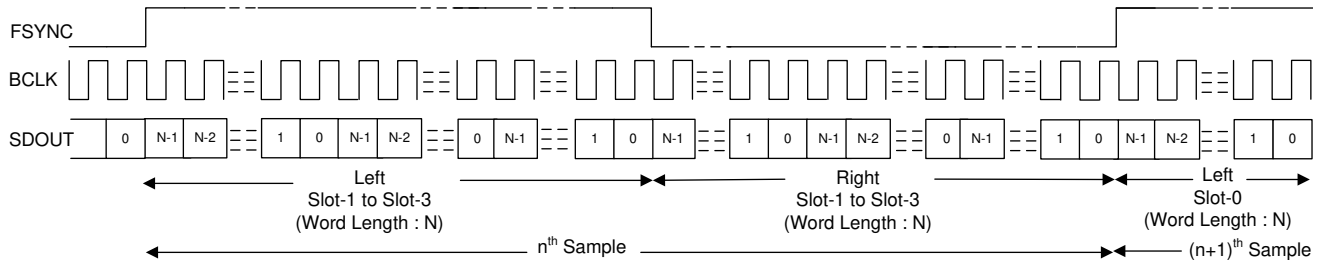
7-11. LJ Protocol Timing (No Idle BCLK Cycles, TX_OFFSET = 0)
