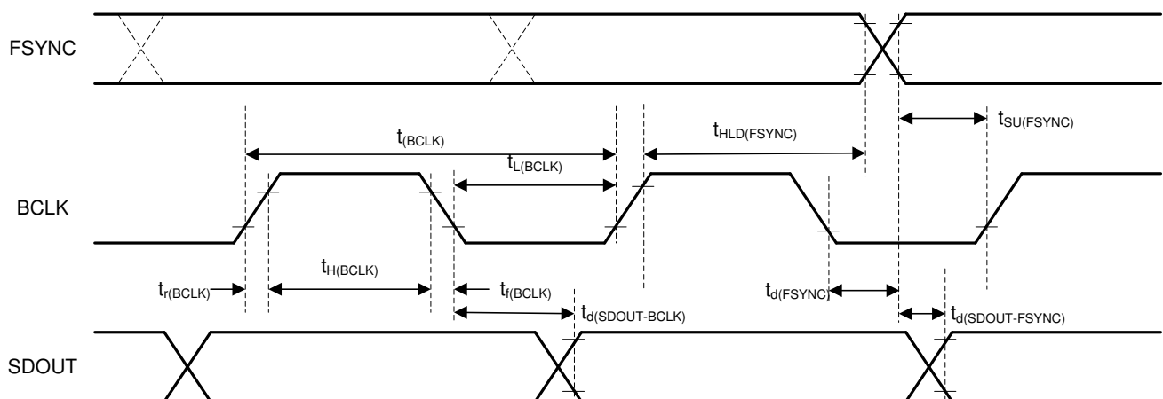
Figure 6-2. TDM (With BCLK_POL = 1), I 2 S, and LJ Interface Timing Diagram
