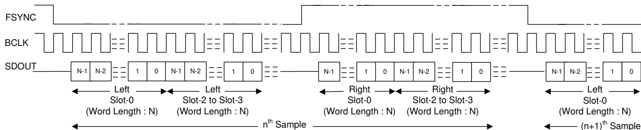
FIG 7-8. I²S Protocol Timing (TX_OFFSET = 0 and BCLK_POL = 1)
