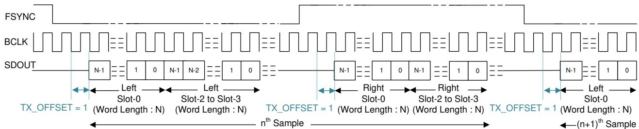
FIG 7-6. I 2 S Protocol Timing (TX_OFFSET = 1)
