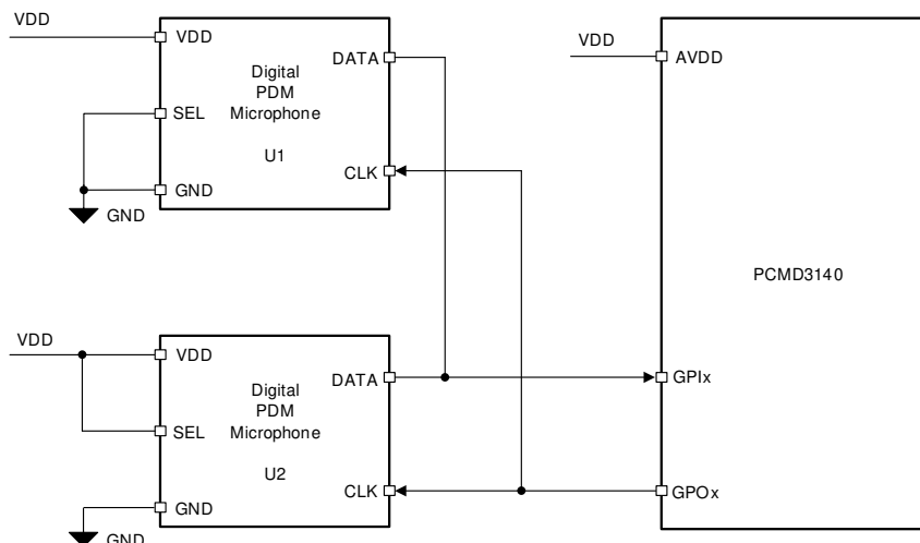
Figure 7-14. Digital PDM Microphones Connection Diagram to the PCMD3140
