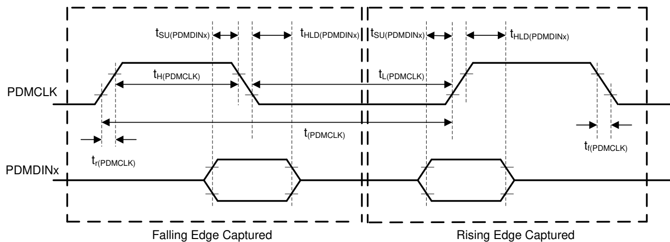
6-3. PDM Digital Microphone Interface Timing Diagram
