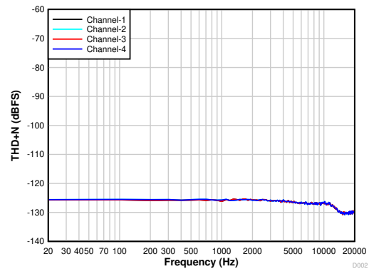
5th-order PDM modulator with PDMCLKx = 3.072\text{ MHz}
