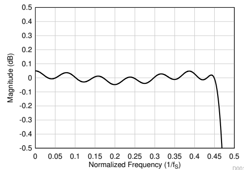
图 7-30. Linear Phase Decimation Filter Pass-Band Ripple
