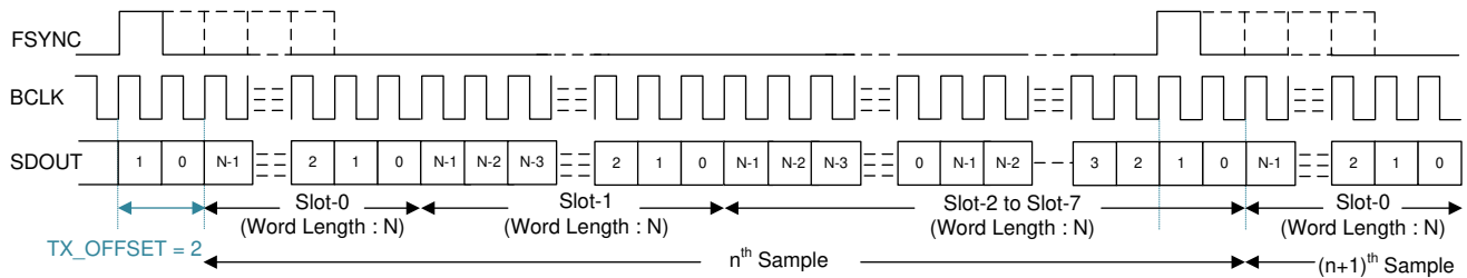
FIG 7-3. TDM Mode Protocol Timing (No Idle BCLK Cycles, TX_OFFSET = 2)
