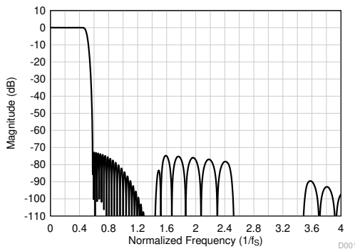
图 7-19. Linear Phase Decimation Filter Magnitude Response
