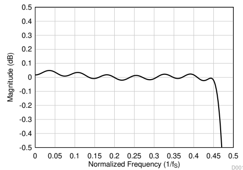
图 7-20. Linear Phase Decimation Filter Pass-Band Ripple
