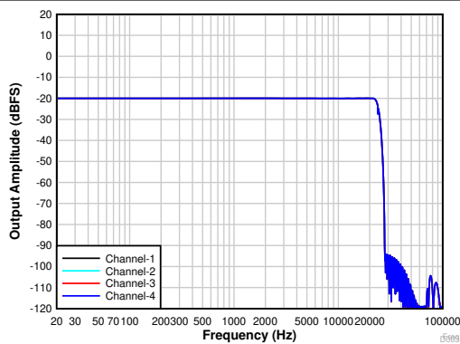
5th-order PDM modulator with PDMCLKx = 3.072\text{ MHz}
