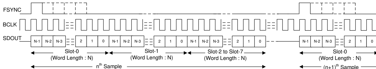
図 7-1. TDM Mode Standard Protocol Timing (TX_OFFSET = 0)
