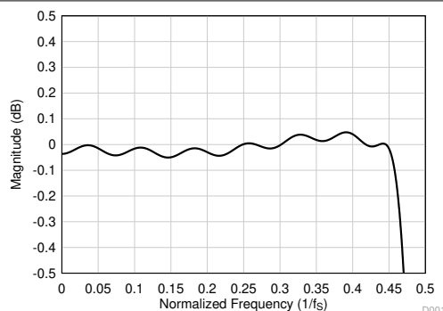
図 7-26. Linear Phase Decimation Filter Pass-Band Ripple
