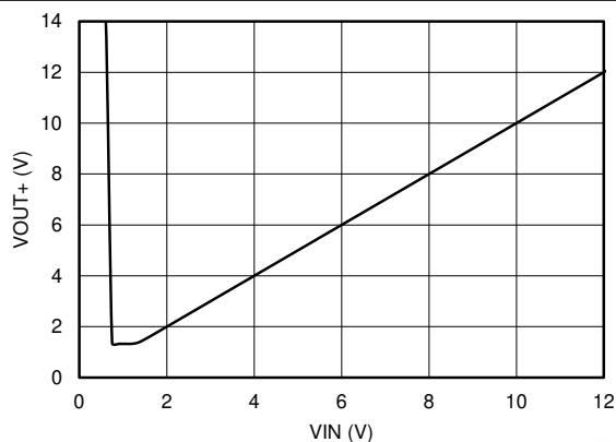
図 7-3. Positive Output Voltage vs Input Voltage
