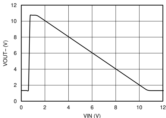
図 7-4. Positive Output Voltage vs Input Voltage
