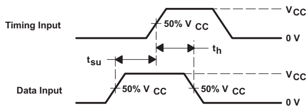
図 6-4. Voltage Waveforms Setup and Hold Times
