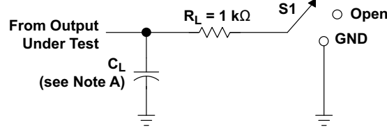
LOAD CIRCUIT FOR 3-STATE AND OPEN-DRAIN OUTPUTS
