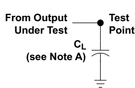
LOAD CIRCUIT FOR TOTEM-POLE OUTPUTS
