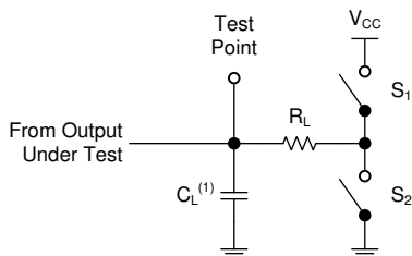
7-1. Load Circuit
