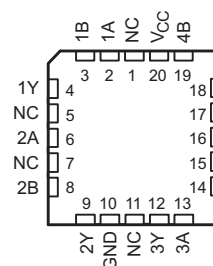
NC - No internal connection 図 4-2. SN54LVC00A FK Package 20-Pin LCCC (Top View)
