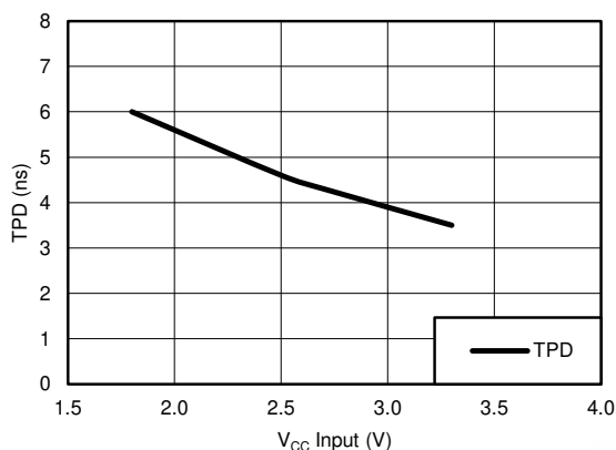
図 5-1. TPD vs V_{CC} ( T_A = 25^\circ\text{C} )
