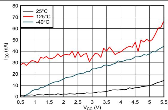
FIG 6-3. Supply Current Across Supply Voltage
