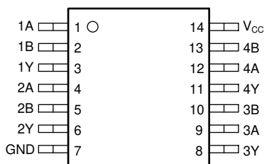
図 5-1. PW Package, 14-Pin TSSOP (Top View)
