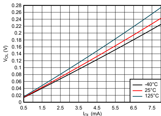
FIG 6-13. Output Voltage vs Current in LOW State; 1.8-V Supply
