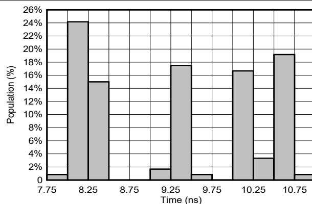
FIG 6-16. T_{PD} Distribution; 2.5-V; T_A = -55^\circ\text{C} to 125^\circ\text{C} (40 Samples)
