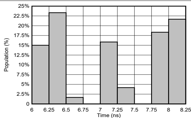
FIG 6-17. T_{PD} Distribution; 3.3-V; T_A = -55^\circ\text{C} to 125^\circ\text{C} (40 Samples)
