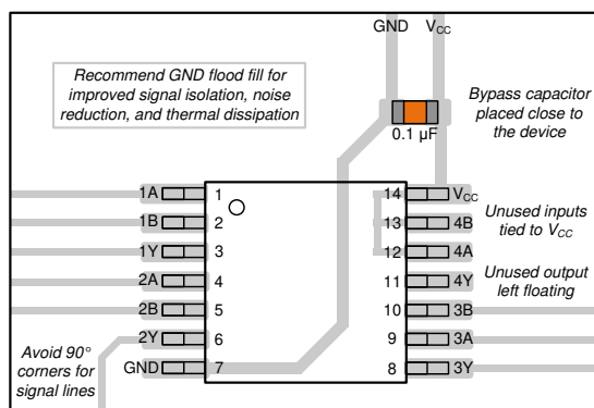
图 9-3. Example Layout for the SN54SC4T08-SEP
