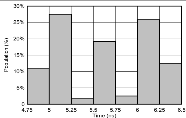
FIG 6-18. T_{PD} Distribution; 5-V; T_A = -55^\circ\text{C} to 125^\circ\text{C} (40 Samples)
