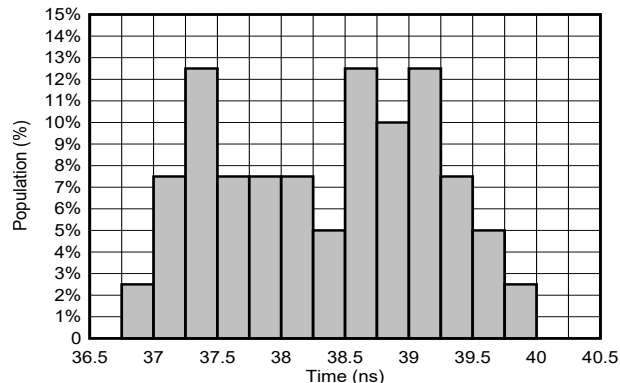
FIG 6-14. T_{PD} Distribution; 1.2-V; T_A = -55^\circ\text{C} to 125^\circ\text{C} (40 Samples)
