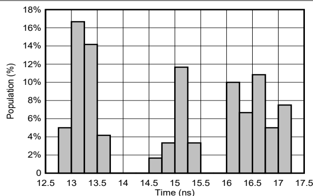
FIG 6-15. T_{PD} Distribution; 1.8-V; T_A = -55^\circ\text{C} to 125^\circ\text{C} (40 Samples)
