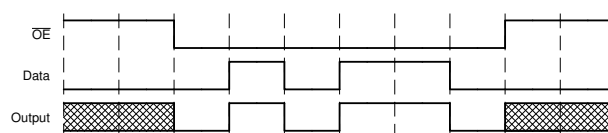
図 8-2. Application Timing Diagram
