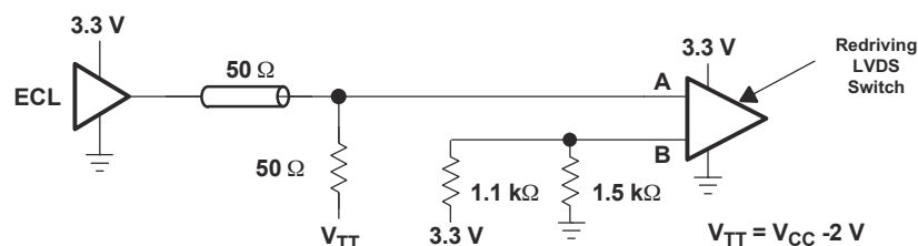
图 9-3. Single-Ended (LVPECL)
