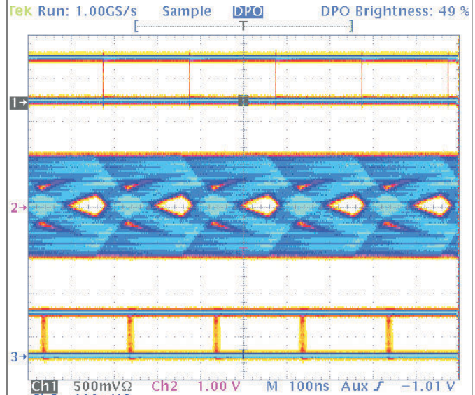
11-3. SN65HVD24 Receiver Performance at 5 Mbps Over 500 Meter Cable
