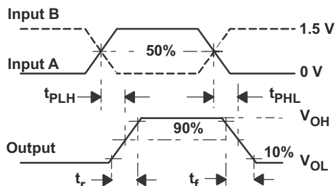
图 7-9. Receiver Switching Test Circuit and Waveforms
