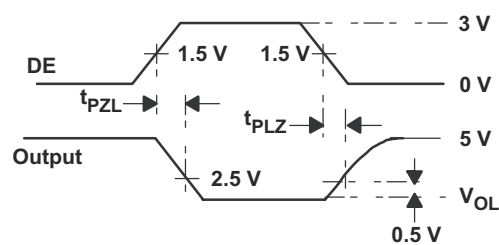
图 7-6. Driver Enable and Disable Test Circuit and Waveforms, Low Output
