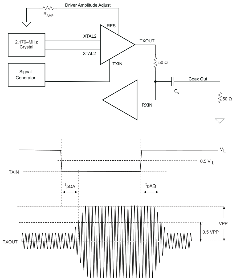
7-1. Measurement of Modem Driver Output Voltage With 50-Ω Loads
