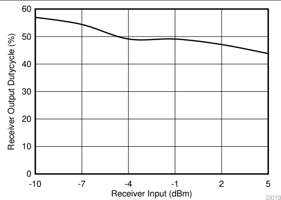
FIG 6-18. Receiver Duty Cycle With 115.2 kbps Signaling Rate
