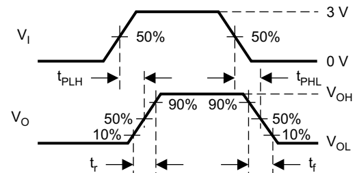
FIG 20. Measurement of Receiver Output Rise and Fall Times and Propagation Delays
