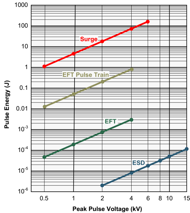
FIG 36. Comparison of Transient Energies
