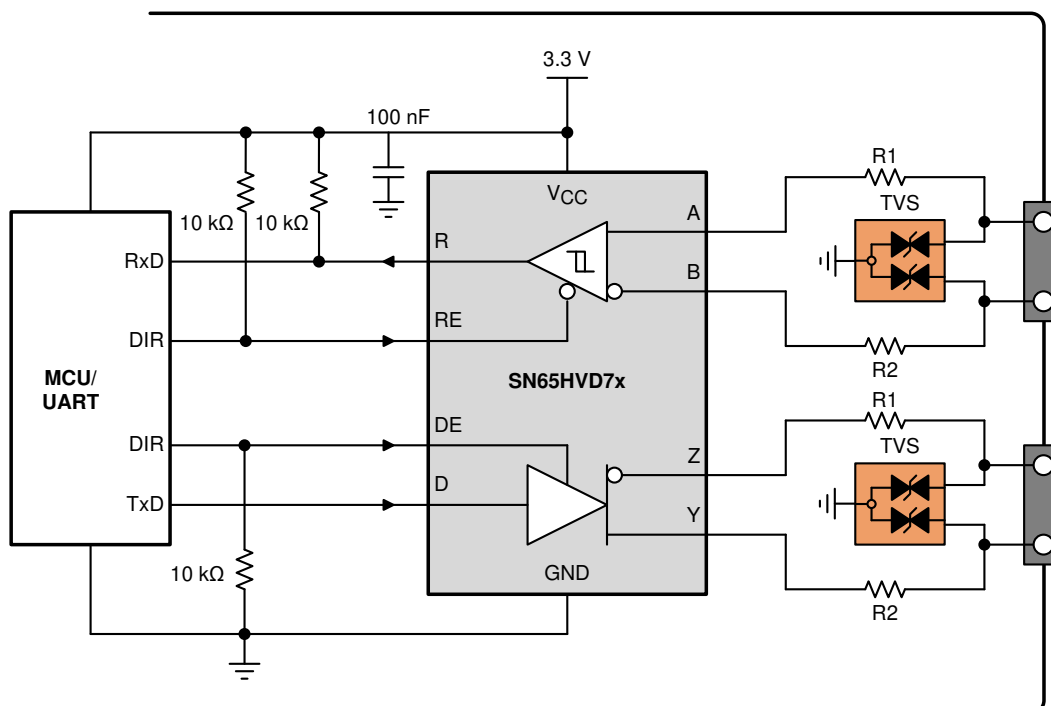
FIG 37. Transient Protection Against ESD, EFT, and Surge transients
