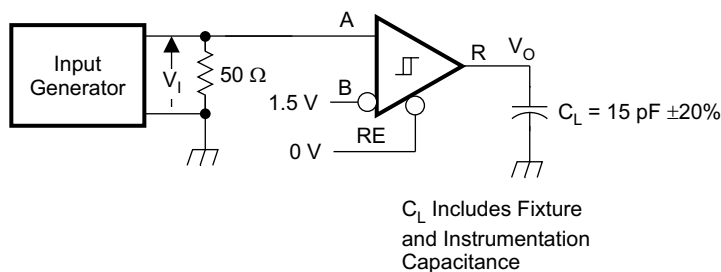
FIG 20. Measurement of Receiver Output Rise and Fall Times and Propagation Delays
