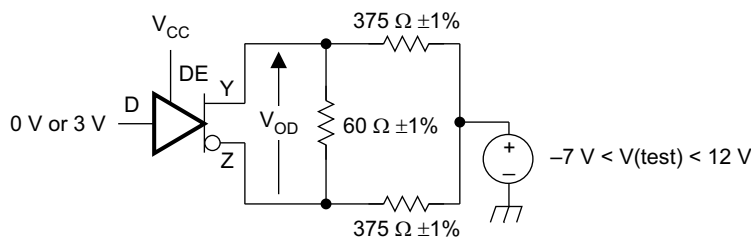
FIG 15. Measurement of Driver Differential Output Voltage With Common-Mode Load
