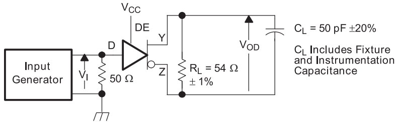
FIG 17. Measurement of Driver Differential Output Rise and Fall Times and Propagation Delays
