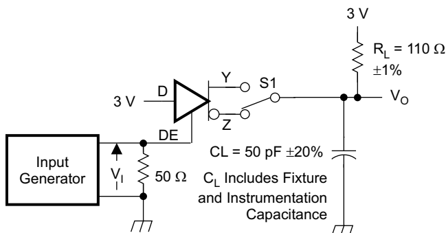
FIG 18. Measurement of Driver Enable and Disable Times with Active-High Output and Pulldown Load
