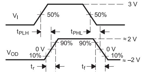
FIG 17. Measurement of Driver Differential Output Rise and Fall Times and Propagation Delays
