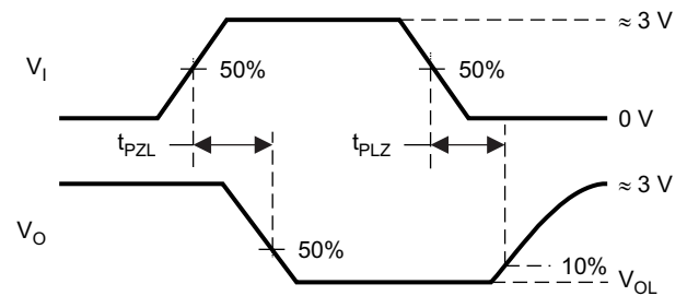
FIG 19. Measurement of Driver Enable and Disable Times with Active-Low Output and Pullup Load
