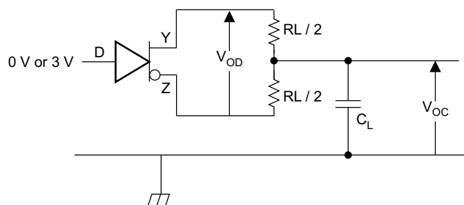
FIG 16. Measurement of Driver Differential and Common-Mode Output With RS-485 Load
