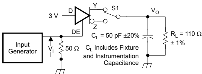
FIG 17. Measurement of Driver Differential Output Rise and Fall Times and Propagation Delays
