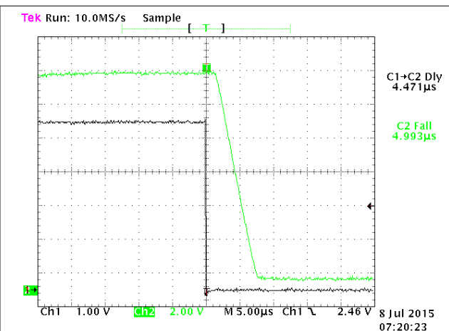
☒ 10-3. Recessive-to-Dominant Propagation Delay
