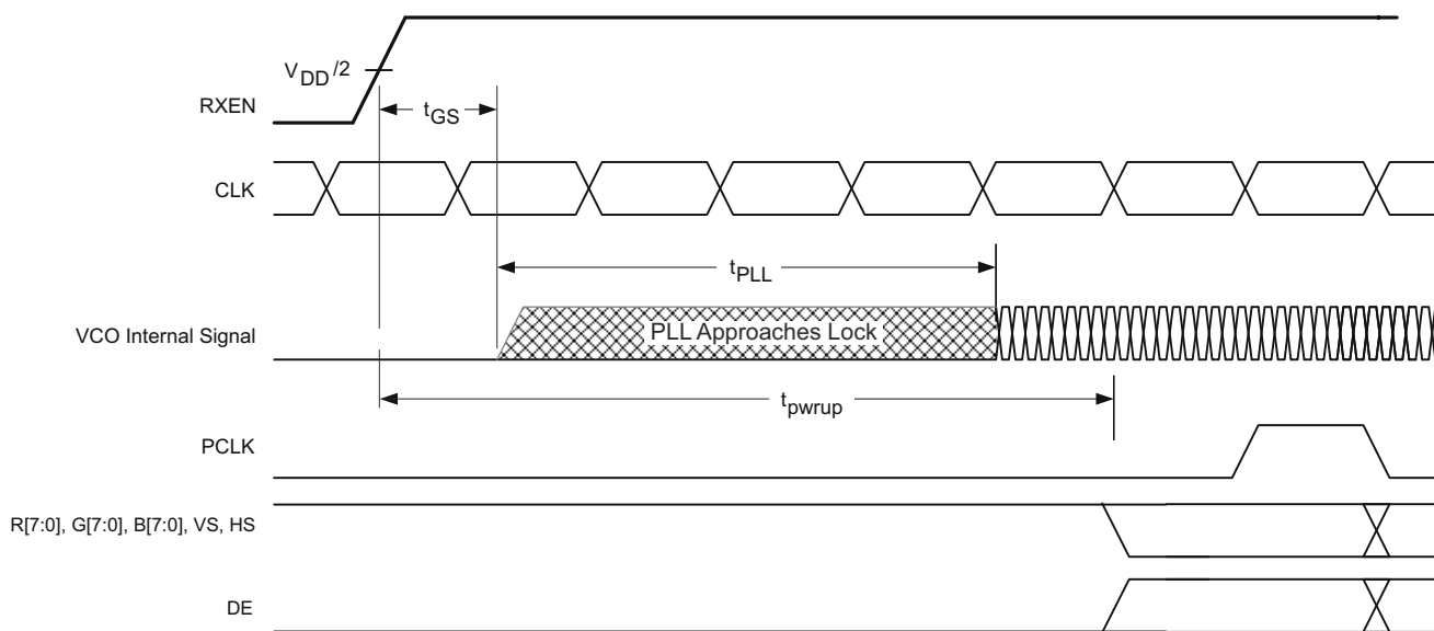
7-9. Receiver Phase Lock Loop Set Time and Receiver Enable Time
