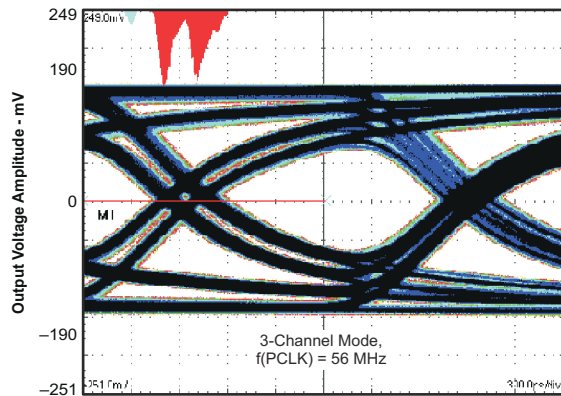
6-12. XGA 3-Channel Output Waveform
