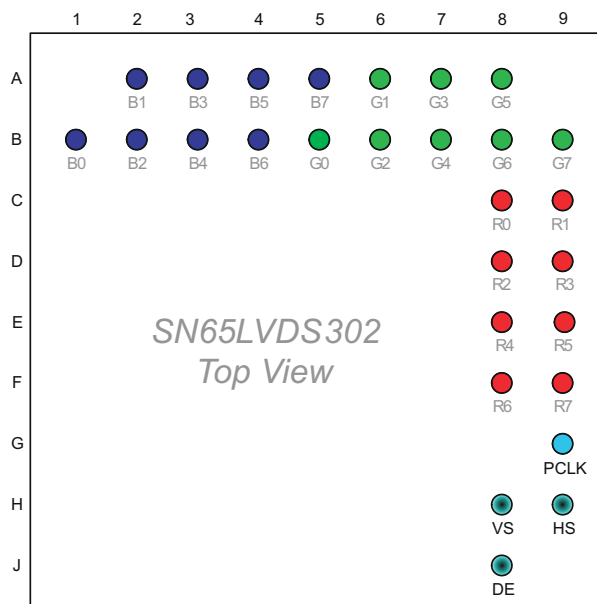
❏ 8-2. Pinout With SWAP PIN = VDD
