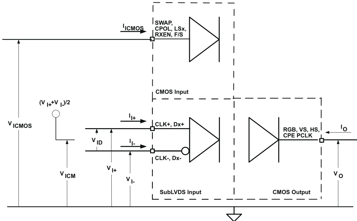
7-6. I/O Voltage and Current Definition
