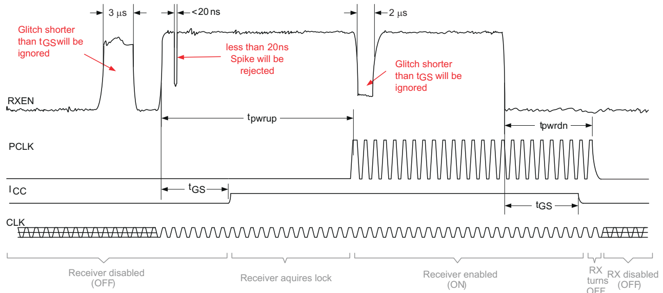
图 7-10. Receiver Enable and Disable Glitch Suppression Time
