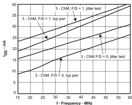
6-5. Supply Current vs Frequency, 3-Channel Mode
