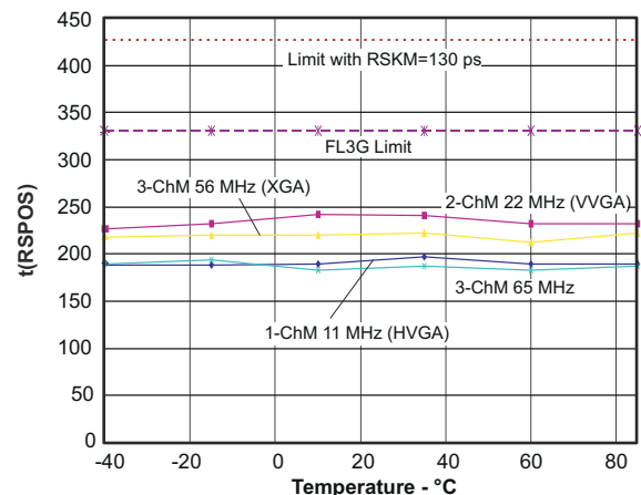
6-6. Receiver Strobe Position vs Temperature
