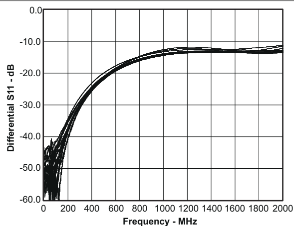
6-15. Input Return Loss
