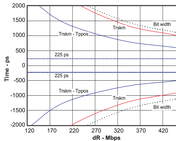
6-10. RSKM, 2-Channel Mode vs Bit Rate
