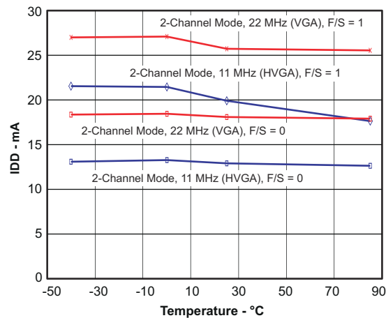
6-1. Supply Current vs Temperature
