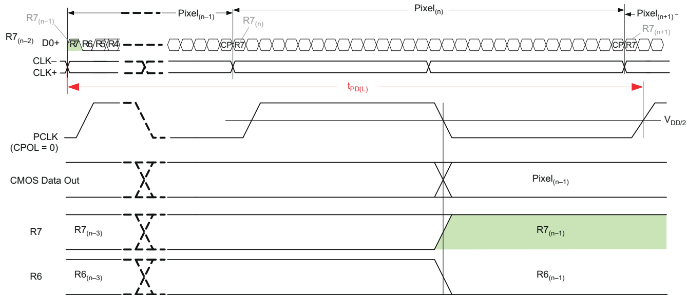
7-8. Propagation Delay Input to Output (LS0 = LS1 = 0)
