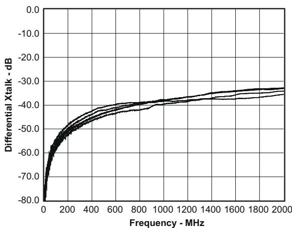
6-16. Input Differential Crosstalk vs Frequency
