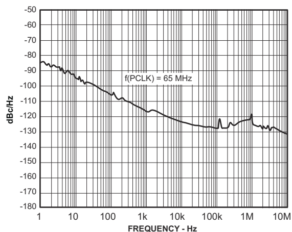
6-17. Phase Noise
