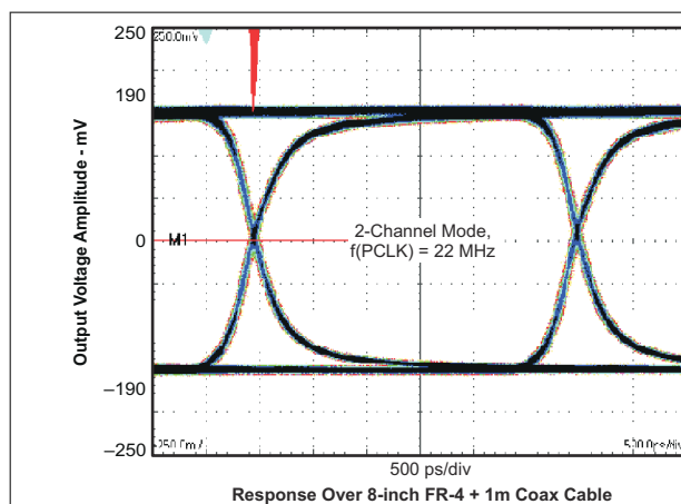
9-6. VGA 2-Channel Output Waveform
