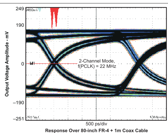
9-7. VGA 2-Channel Output Waveform
