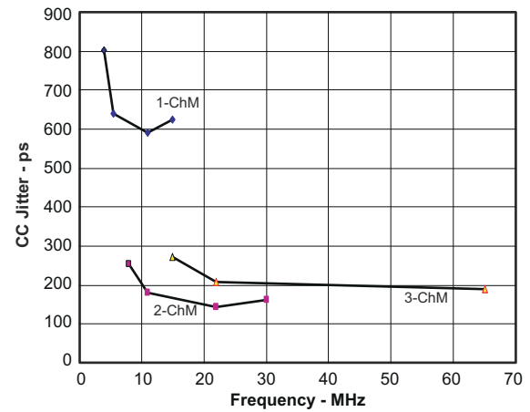
6-8. PCLK Cycle-to-Cycle Output Jitter
