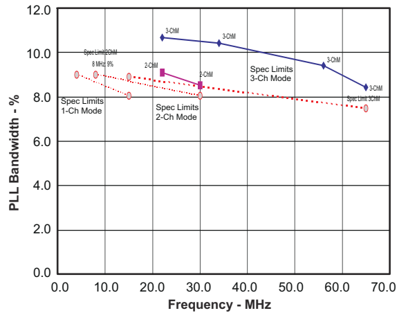
6-7. PLL Bandwidth
