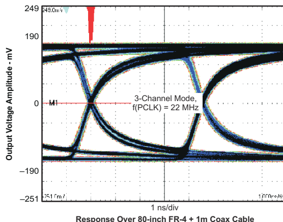
9-8. VGA3-Channel Output Waveform
