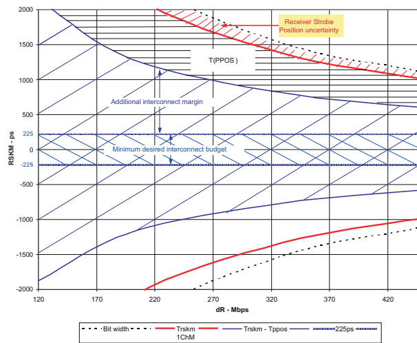
6-9. RSKM, 1-Channel Mode vs Bit Rate
