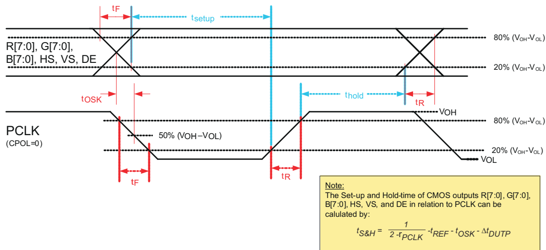
7-3. Output Rise and Fall, Setup and Hold Time
