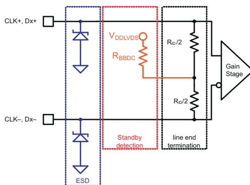
7-5. Equivalent Input Circuit Design
