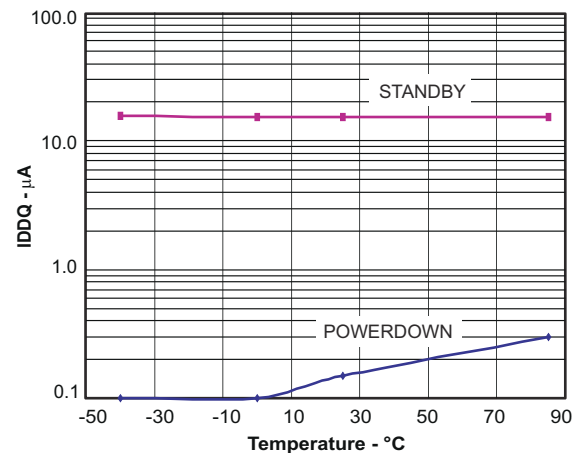
6-2. Quiescent Supply Current vs Temperature
