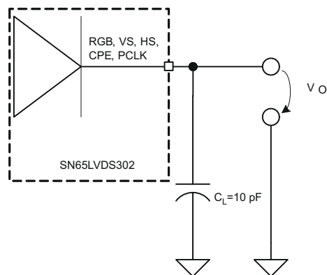
7-7. CMOS Output Test Circuit, Signal and Timing Definition
