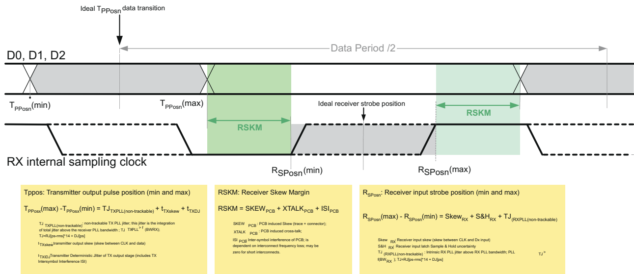
9-2. Jitter Budget
