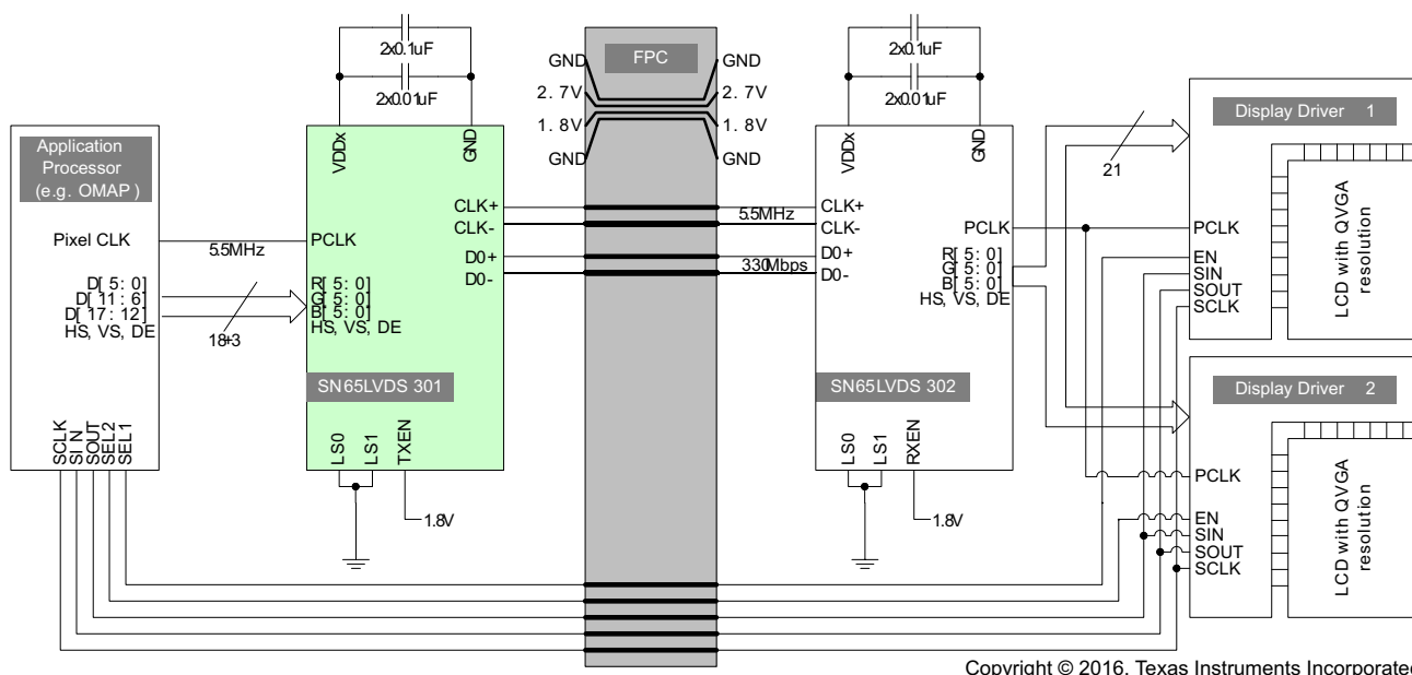
9-9. Example Dual-QVGA Display Application
