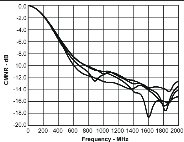
6-14. Input Common-Mode Noise Rejection vs Frequency
