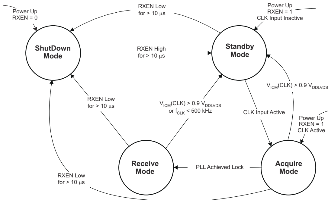
8-7. Operating Modes and State Machine Diagram
