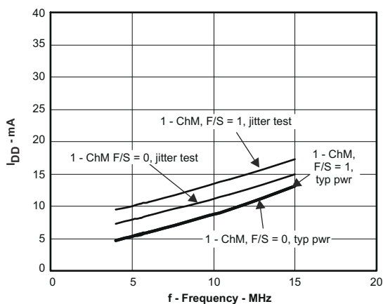
6-3. Supply Current vs Frequency, 1-Channel Mode
