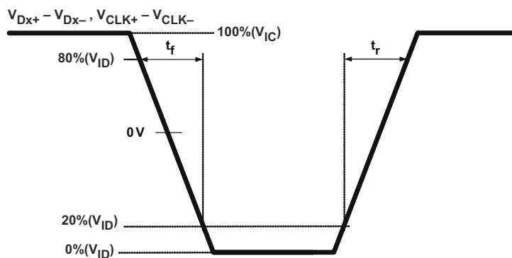
7-4. SubLVDS Differential Input Rise and Fall Time Definition
