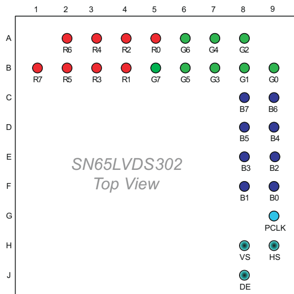
❏ 8-1. Pinout With SWAP PIN = GND
