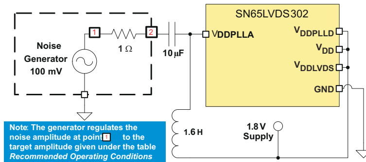
7-1. Power Supply Noise Test Set-Up
