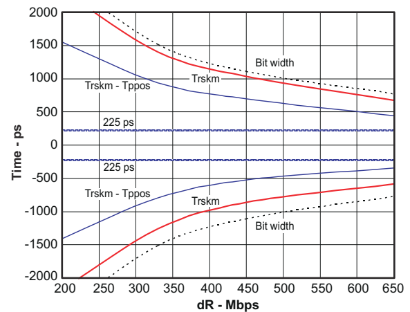
6-11. RSKM, 3-Channel Mode vs Bit Rate
