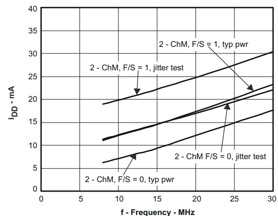
6-4. Supply Current vs Frequency, 2-Channel Mode
