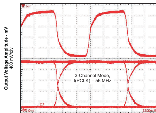
6-13. XGA 3-Channel Output Waveform
