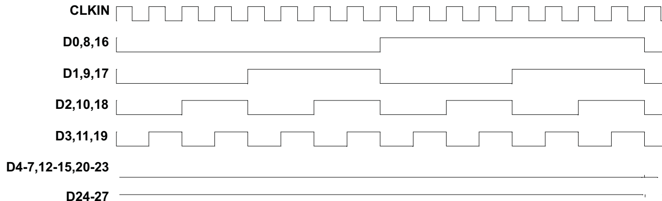
FIG 8. 16 Grayscale Test Pattern
