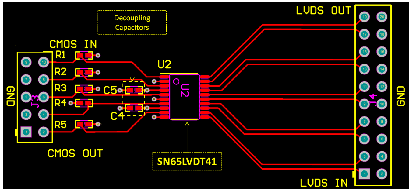
Figure 33. Example SN65LVDT41
