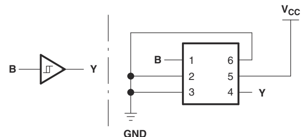
图 7-10. 17/34: Noninverted Buffer
