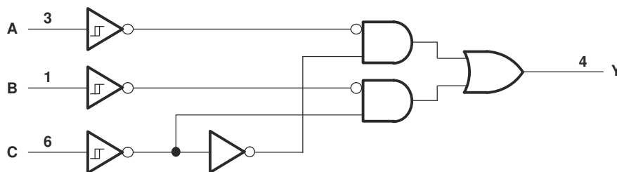
FIG 7-1. Logic Diagram (Positive Logic)
