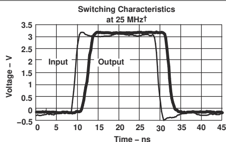
5-2. Excellent Signal Integrity
