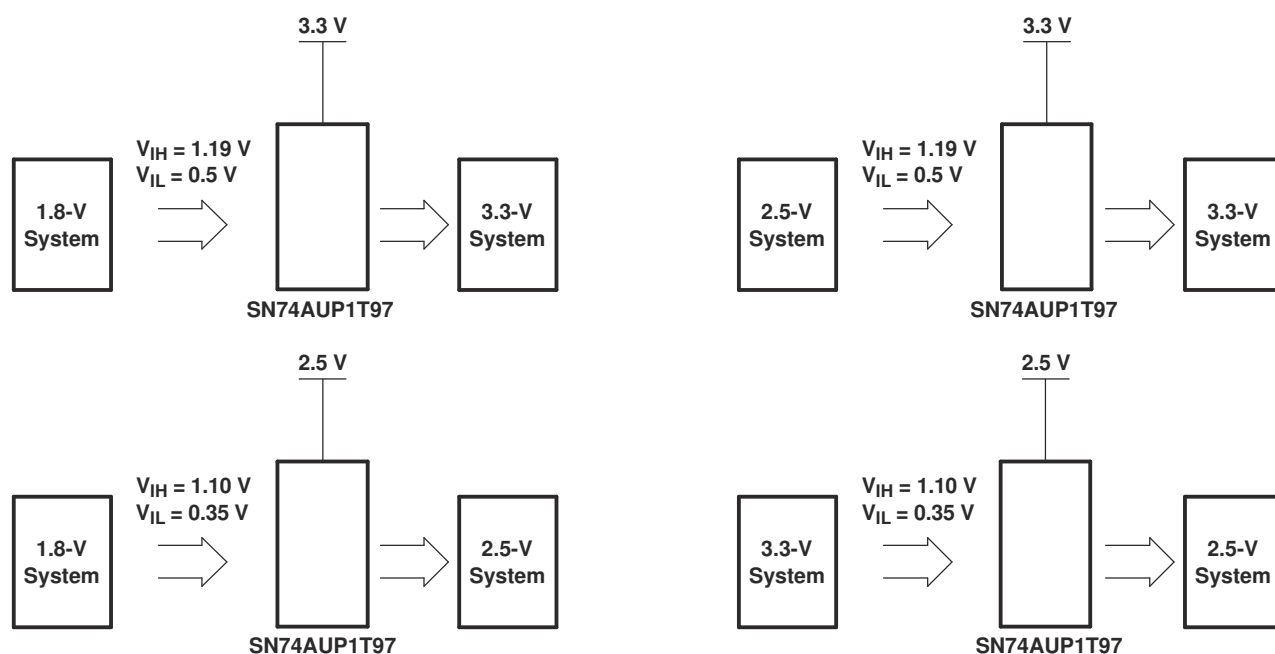
FIG 7-2. Possible Voltage-Translation Combinations
