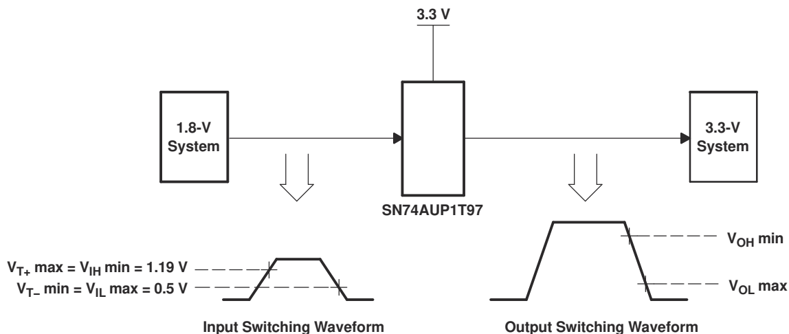
FIG 7-3. Switching Thresholds for 1.8-V to 3.3-V Translation
