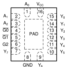
BQB Package 16-Pin WQFN Top View
