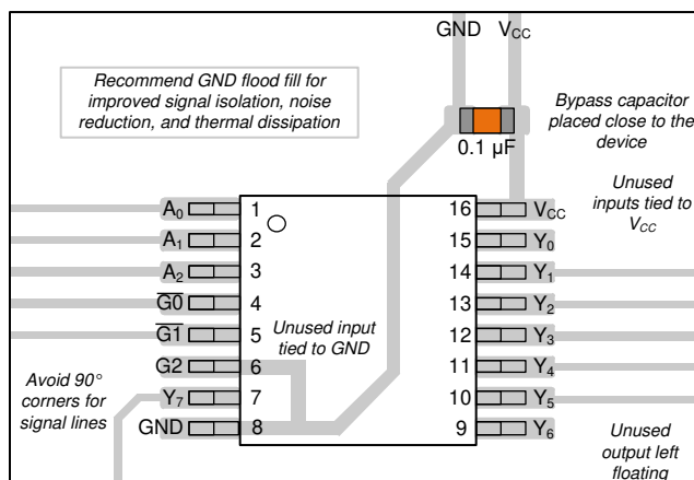
✎ 11-1. Example layout for the SN74HCS238-Q1.
