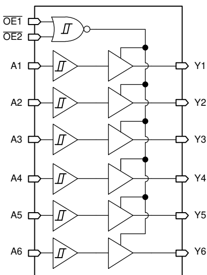
FIG 8-1. Logic Diagram (Positive Logic) for SN74HCS365-Q1
