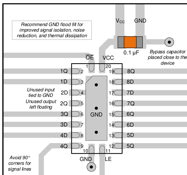
11-1. Example Layout for the SN74HCS373-Q1 in the WRKS Package
