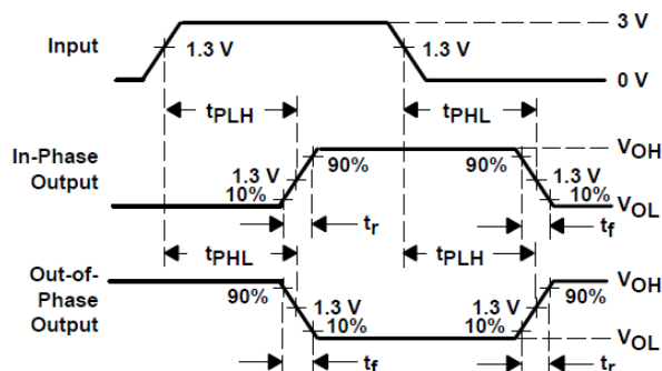
图 6-4. Voltage Waveforms Propagation Delay and Output Rise and Fall Times
