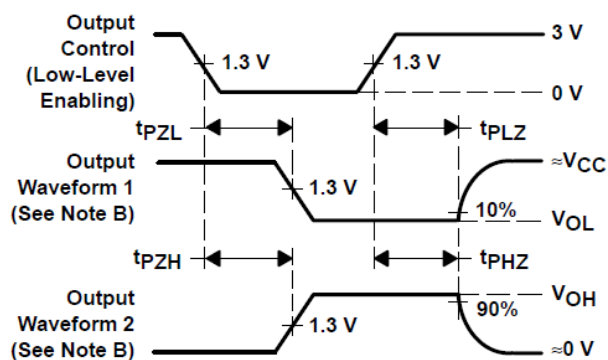
图 6-5. Voltage Waveforms Enable and Diable Times for 3-State Outputs
