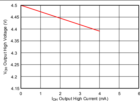
6-2. Typical Output Voltage in the High State ( V_{OH} )
