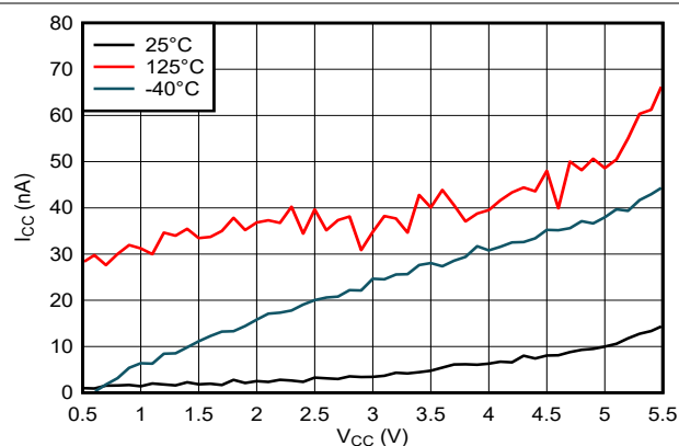
図 5-3. Supply Current Across Supply Voltage
