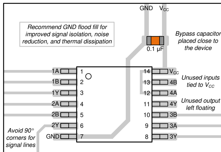
図 10-1. Example Layout for the SN74LV4T00-EP
