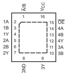
図 3-2. BQB Package, 16-Pin WQFN with Exposed Thermal Pad (Top View)
