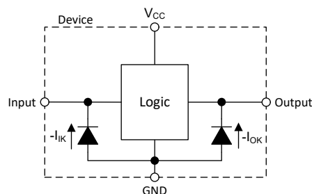
✎ 7-1. Electrical Placement of Clamping Diodes for Each Input and Output
