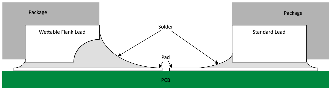
✎ 7-2. Simplified Cutaway View of Wettable-Flank QFN Package and Standard QFN Package After Soldering
