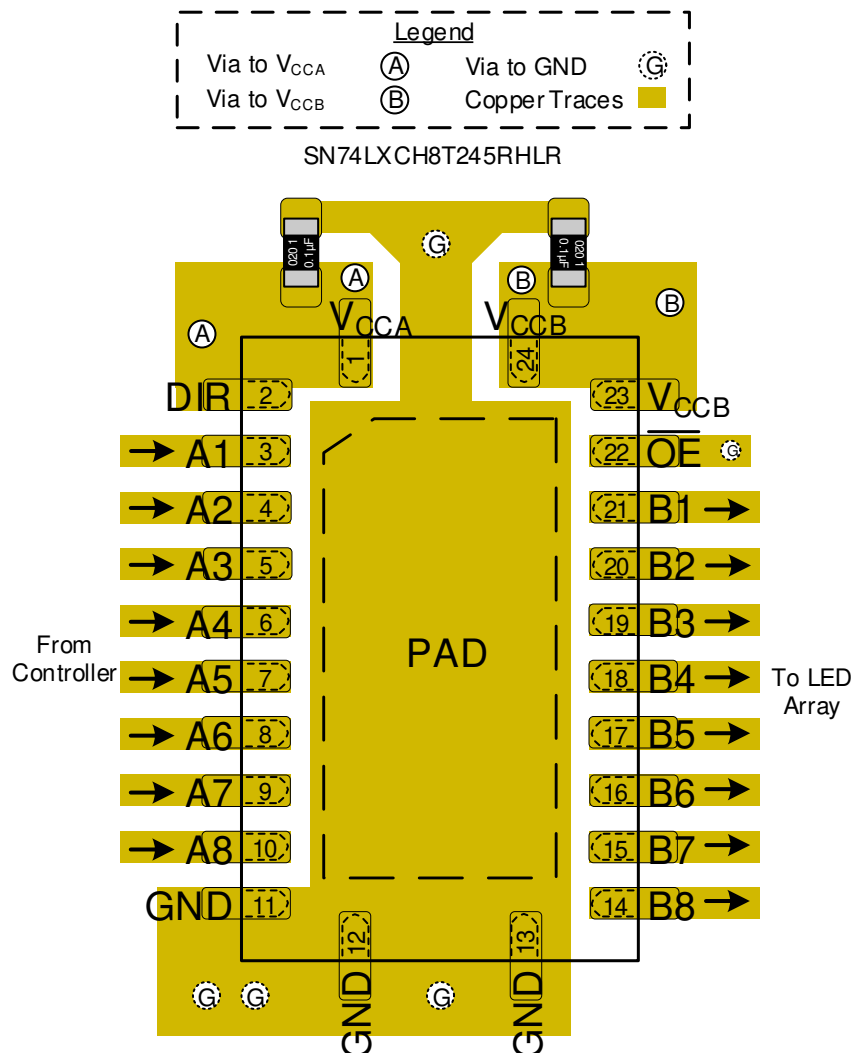
11-1. Layout Example
