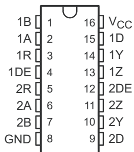
図 4-2. SN65C1168: N, NS, or PW Package SN75C1168: DB, N, NS, or PW Package (Top View)
