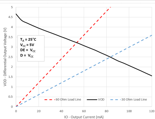
5-11. Differential Output Voltage vs Differential Output Current
