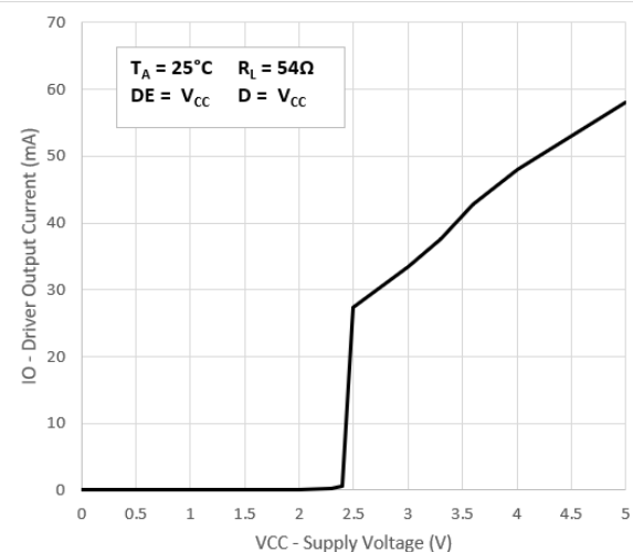
5-10. Driver Output Current vs Supply Voltage
