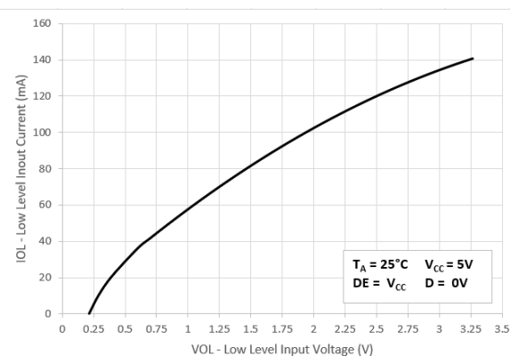
5-8. Driver Low-Level Output Current vs Low-Level Output Voltage
