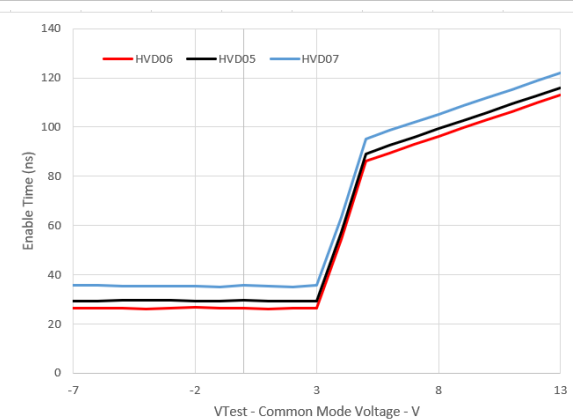
5-12. Enable Time vs Common-Mode Voltage (See 5-13)
