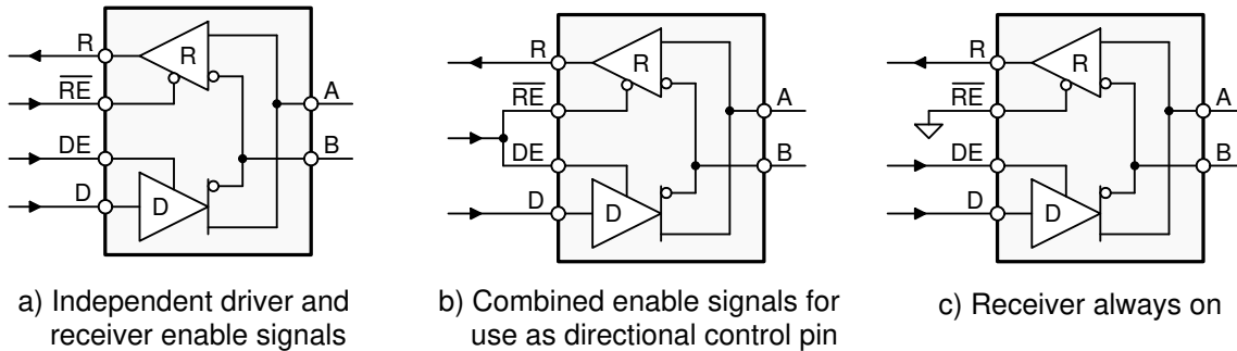
図 10-1. Half-Duplex Transceiver Configurations
