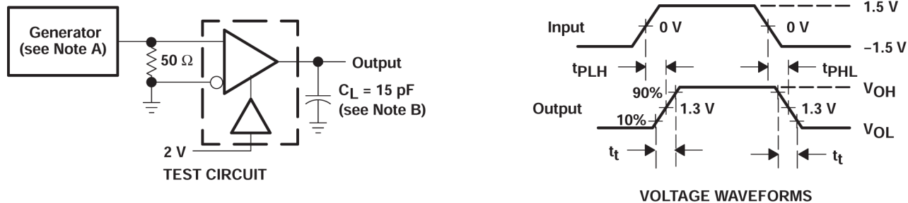
図 6-1. t_{PLH} and t_{PHL} Test Circuit and Voltage Waveforms
