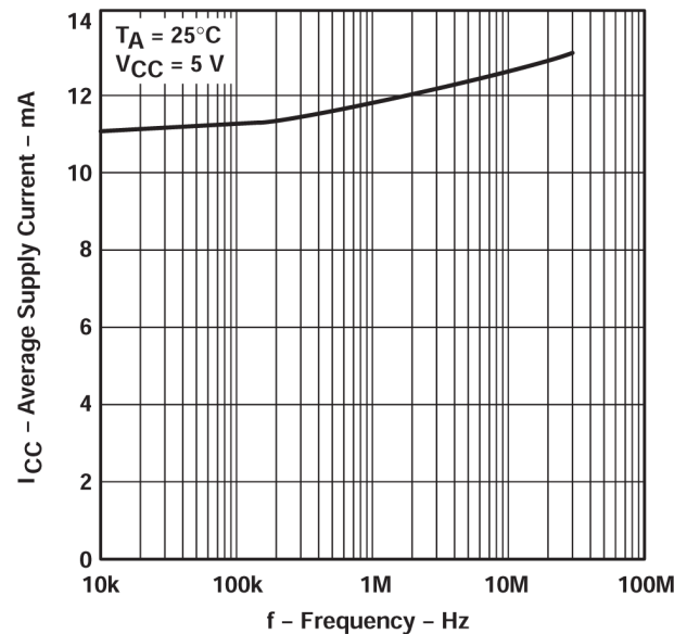
図 5-4. Average Supply Current vs Frequency
