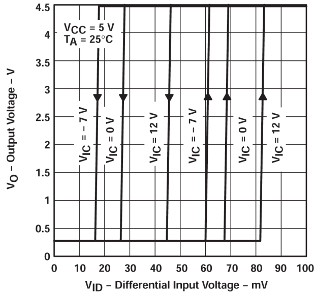
図 5-1. Output Voltage vs Differential Input Voltage
