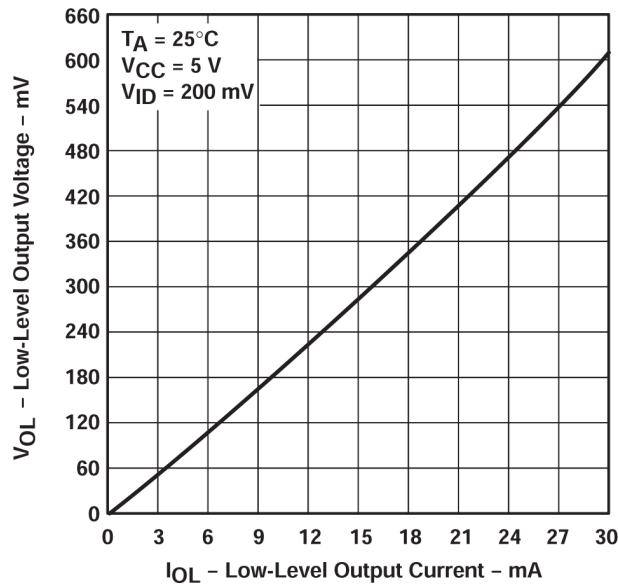
図 5-3. Low-level Output Voltage vs Low-level Output Current
