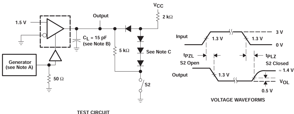
図 6-2. t_{PHZ} and t_{PZH} Test Circuit and Voltage Waveforms
