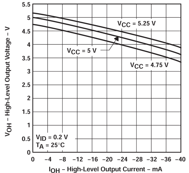
図 5-2. High-level Output Voltage vs High-level Output Current
