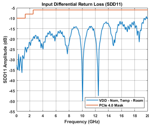
Figure 6-3. Typical Input (RX) Differential Return Loss vs Frequency in TI Evaluation Board with \approx 2 dB input and \approx 2 dB Output Loss
