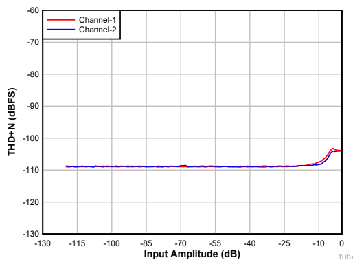
Differential output
