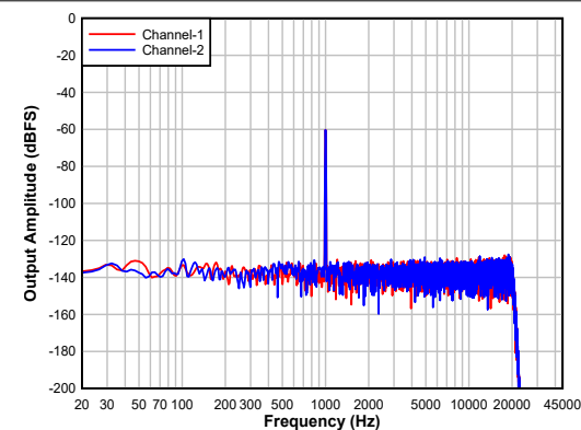
6-9. ADC Frequency Response
