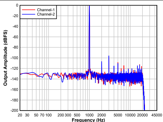
6-10. ADC FFT with Idle Channel Input
