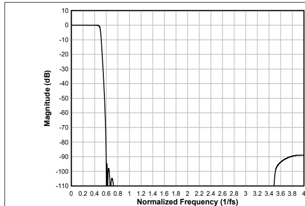
図 6-40. Low-latency Interpolation Filter Magnitude Response
