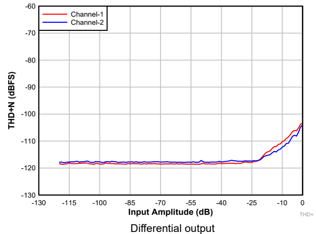
图 8-3. DAC THD+N Level vs Input
