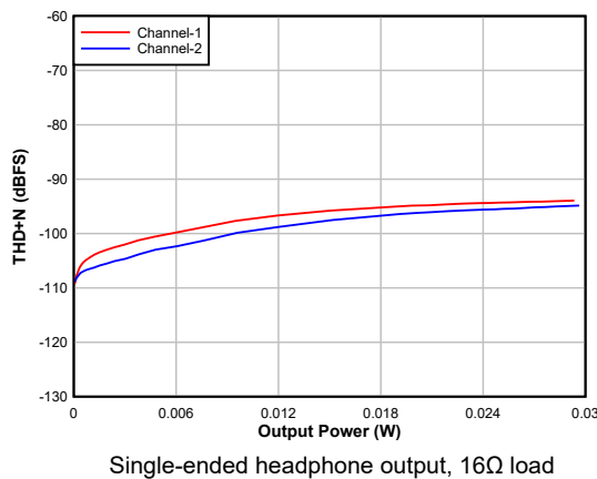
図 5-9. DAC THD+N Level vs output power
