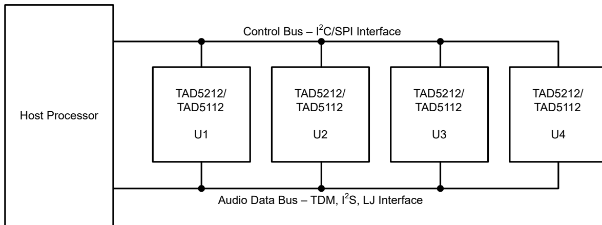
图 6-13. Multiple TAD5212 Devices With Shared Control and Audio Data Buses
