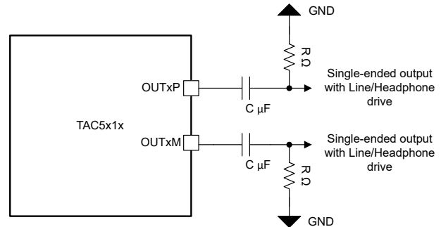
図 6-17. Stereo Single-ended Output Connection (OUT1x_CFG[2:0] = 3'b001)
