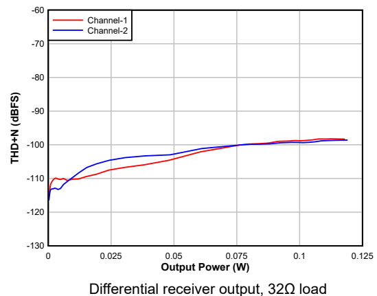
図 5-8. DAC THD+N Level vs output power
