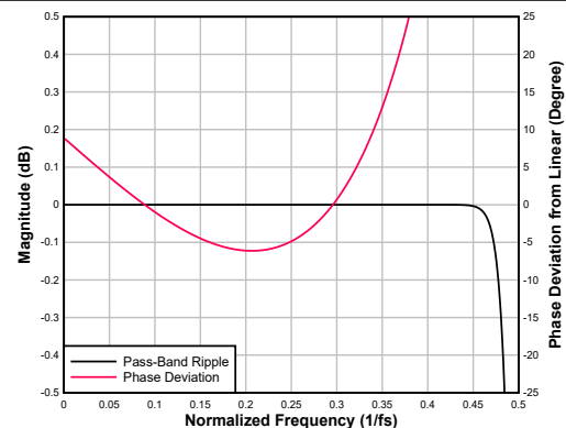
図 6-59. Ultra-Low-Latency interpolation Filter Pass-Band Ripple and Phase Deviation
