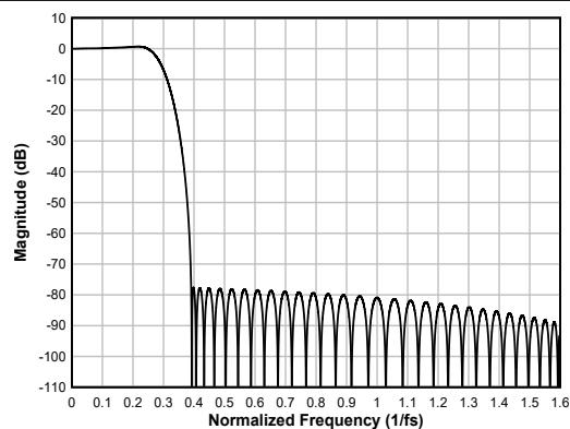
図 6-36. Linear-phase Interpolation Filter Magnitude Response
