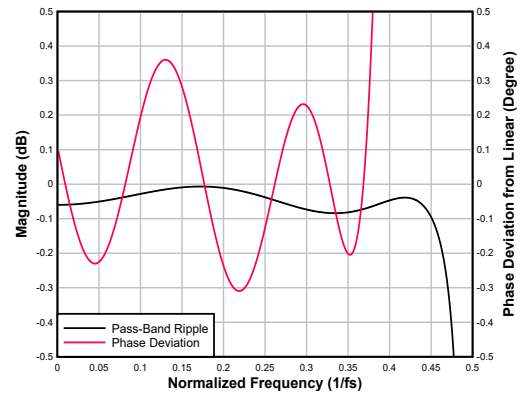
図 6-45. Low-latency Interpolation Filter Pass-Band Ripple and Phase Deviation
