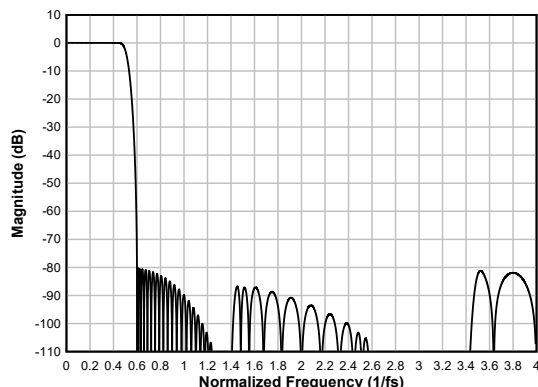
図 6-64. Linear-phase Decimation Filter Magnitude Response
