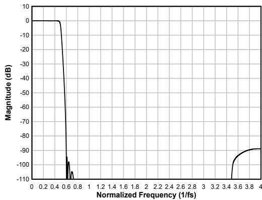
図 6-44. Low-latency Interpolation Filter Magnitude Response
