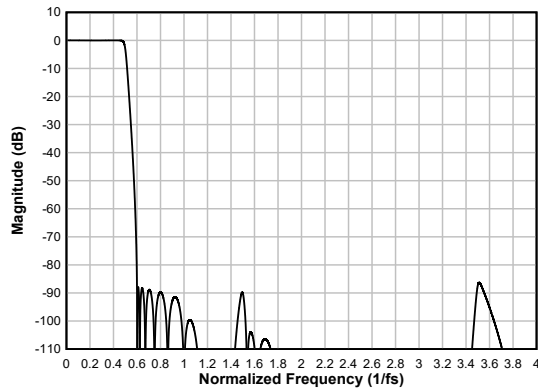
図 6-94. Ultra Low-latency Decimation Filter Magnitude Response
