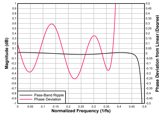
図 6-85. Low-latency Decimation Filter Pass-Band Ripple and Phase Deviation
