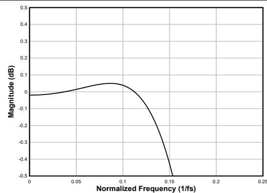
図 6-79. Linear-phase Decimation Filter Pass-Band Ripple
