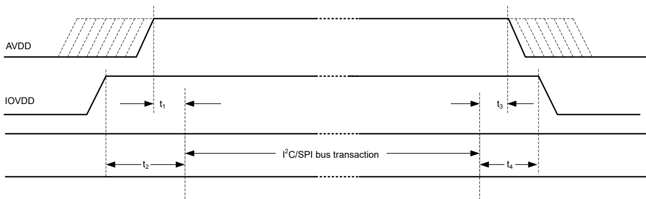
図 8-4. Power-Supply Sequencing Requirement Timing Diagram
