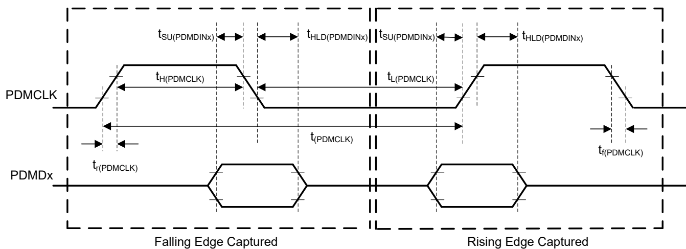
図 5-4. PDM Digital Microphone Interface Timing Diagram
