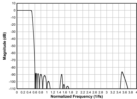
図 6-84. Low-latency Decimation Filter Magnitude Response
