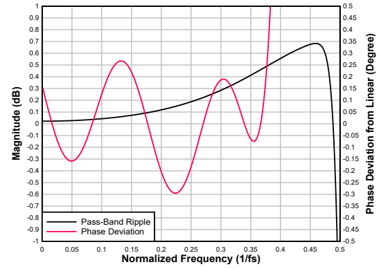
図 6-81. Low-latency Decimation Filter Pass-Band Ripple and Phase Deviation
