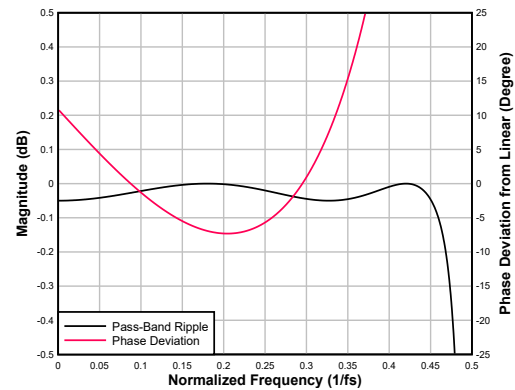
図 6-57. Ultra-Low-Latency interpolation Filter Pass-Band Ripple and Phase Deviation
