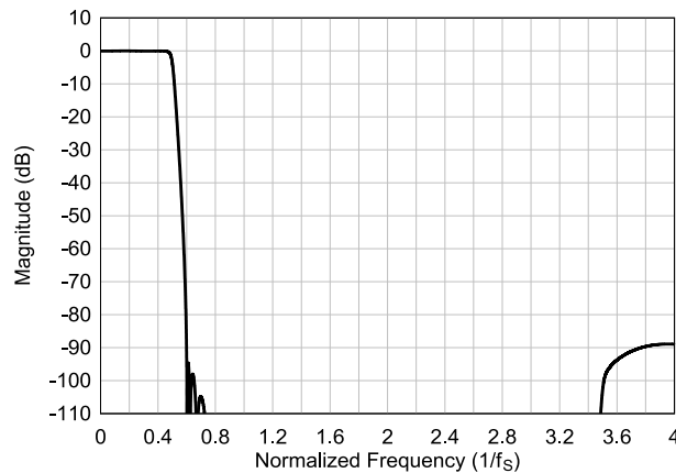
図 6-50. Ultra-Low-Latency interpolation Filter Magnitude Response
