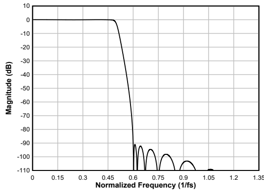
図 6-88. Low-latency Decimation Filter Magnitude Response
