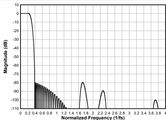
図 6-76. Linear-phase Decimation Filter Magnitude Response
