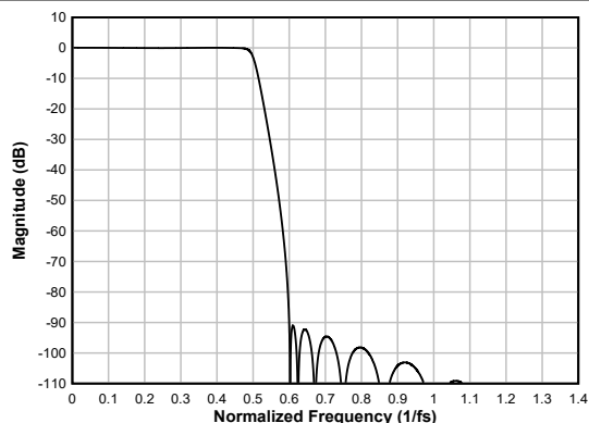
6-98. Ultra Low-latency Decimation Filter Magnitude Response
