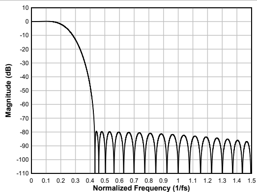
図 6-38. Linear-phase Interpolation Filter Magnitude Response
