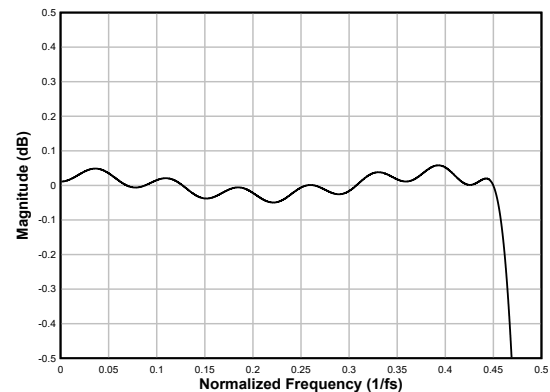
図 6-73. Linear-phase Decimation Filter Pass-Band Ripple
