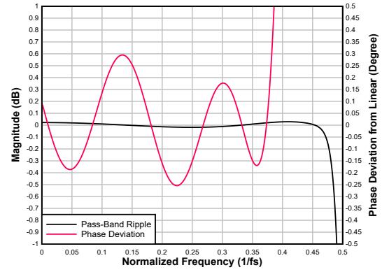
図 6-87. Low-latency Decimation Filter Pass-Band Ripple and Phase Deviation
