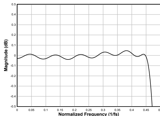
図 6-67. Linear-phase Decimation Filter Pass-Band Ripple
