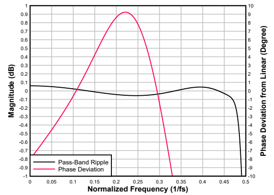
図 6-89. Low-latency Decimation Filter Pass-Band Ripple and Phase Deviation
