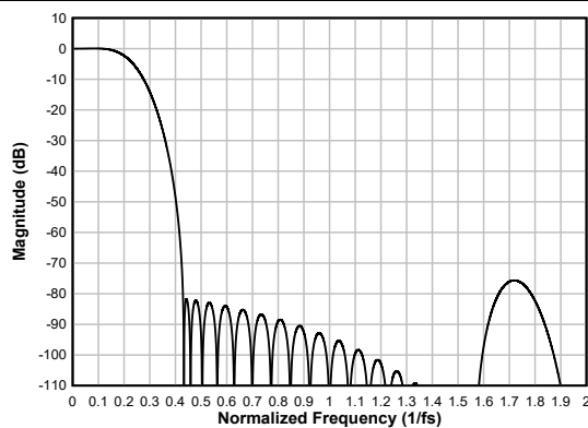
図 6-78. Linear-phase Decimation Filter Magnitude Response
