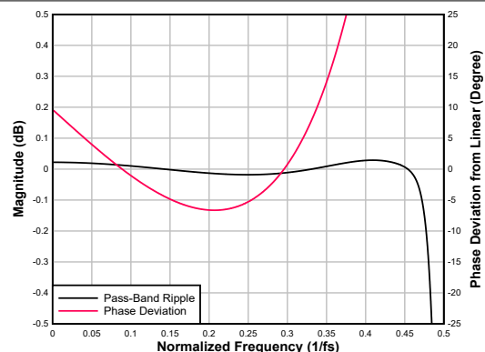
図 6-97. Ultra Low-latency Decimation Filter Pass-Band Ripple and Phase Deviation
