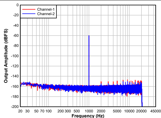
Differential output
