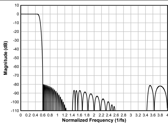
図 6-62. Linear-phase Decimation Filter Magnitude Response
