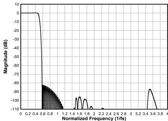
図 6-72. Linear-phase Decimation Filter Magnitude Response
