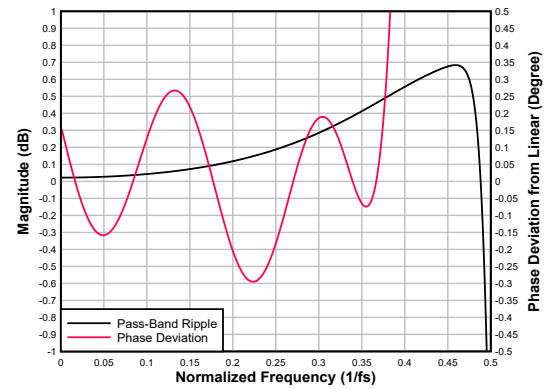
図 6-83. Low-latency Decimation Filter Pass-Band Ripple and Phase Deviation
