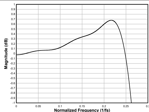
図 6-37. Linear-phase Interpolation Filter Pass-Band Ripple
