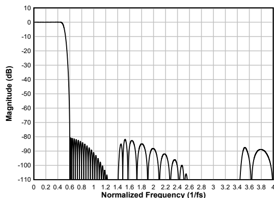
図 6-66. Linear-phase Decimation Filter Magnitude Response
