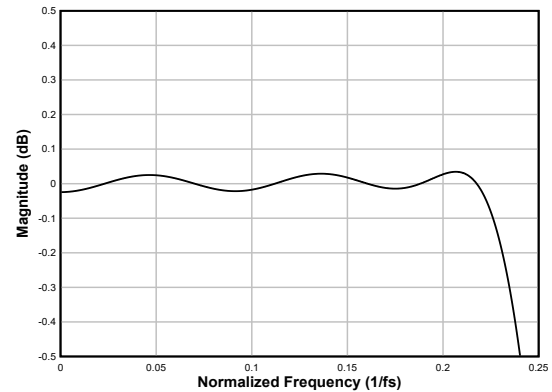
図 6-75. Linear-phase Decimation Filter Pass-Band Ripple
