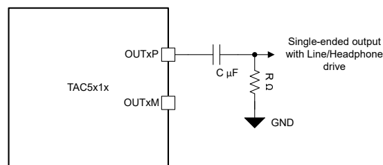
図 6-15. Mono Single-ended Output Connection on OUT1P (OUT1x_CFG[2:0] = 3'b010)
