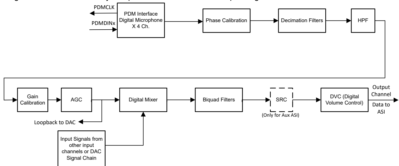
FIG 6-60. PDM Recording Signal-Chain Processing Flowchart
