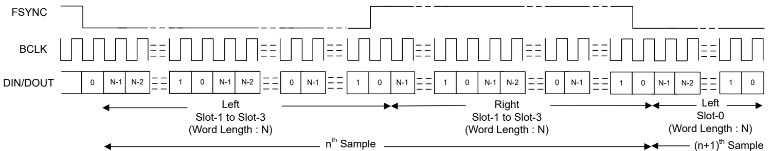
図 6-7. I 2 S Protocol Timing (No Idle BCLK Cycles, PASI_TX_OFFSET = 0)
