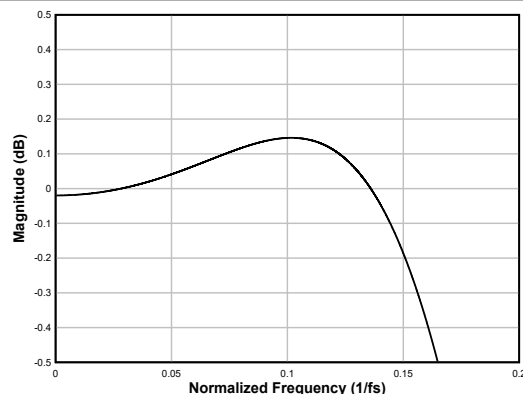
図 6-39. Linear-phase Interpolation Filter Pass-Band Ripple
