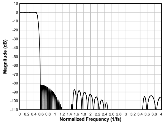
図 6-26. Linear-phase Interpolation Filter Magnitude Response
