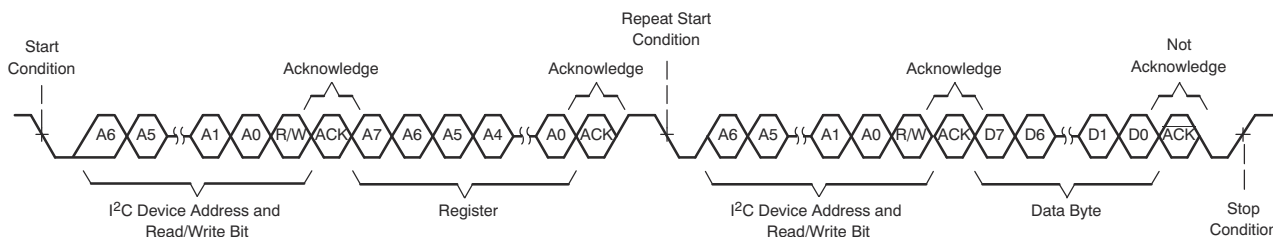
Figure 6-104. I 2 C Single-Byte Read Transfer
