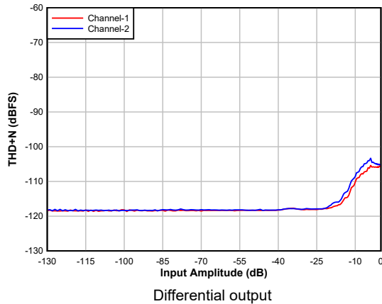
図 5-5. DAC THD+N Level vs Input
