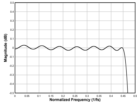
図 6-27. Linear-phase Interpolation Filter Pass-Band Ripple
