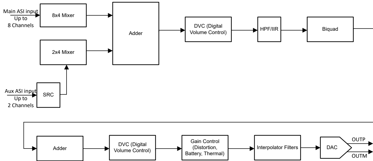
Figure 6-20. DAC Signal-Chain Processing Flowchart
