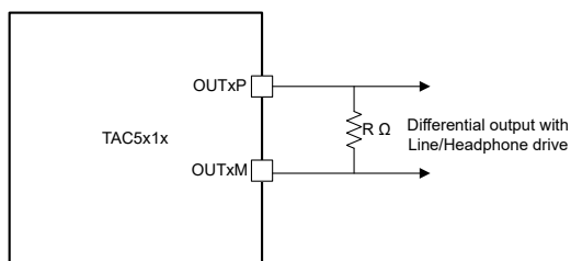
図 6-14. Differential Output Connection (OUT1x_CFG[2:0] = 3'b000)
