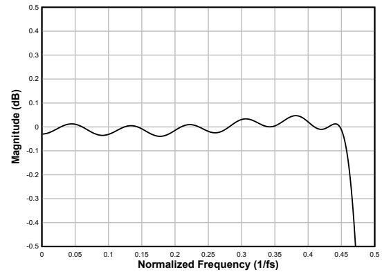
図 6-69. Linear-phase Decimation Filter Pass-Band Ripple
