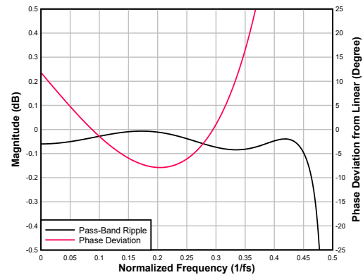
図 6-51. Ultra-Low-Latency interpolation Filter Pass-Band Ripple and Phase Deviation
