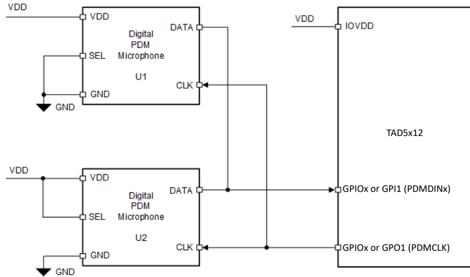
図 6-18. Digital PDM Microphones Connection Diagram for the TAD5212
