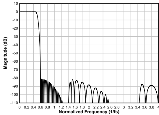
図 6-68. Linear-phase Decimation Filter Magnitude Response
