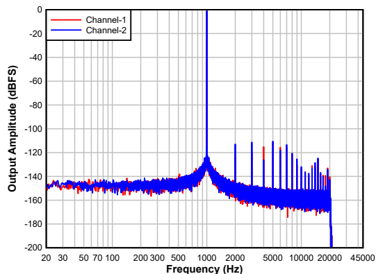
Figure 5-17. DAC FFT with -1dBFS Input
