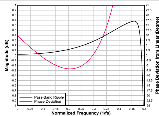
図 6-91. Ultra Low-latency Decimation Filter Pass-Band Ripple and Phase Deviation
