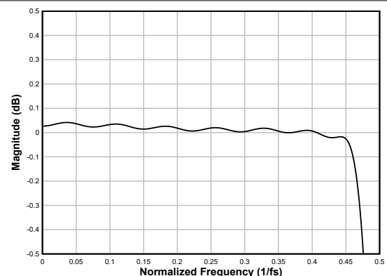
図 6-63. Linear-phase Decimation Filter Pass-Band Ripple
