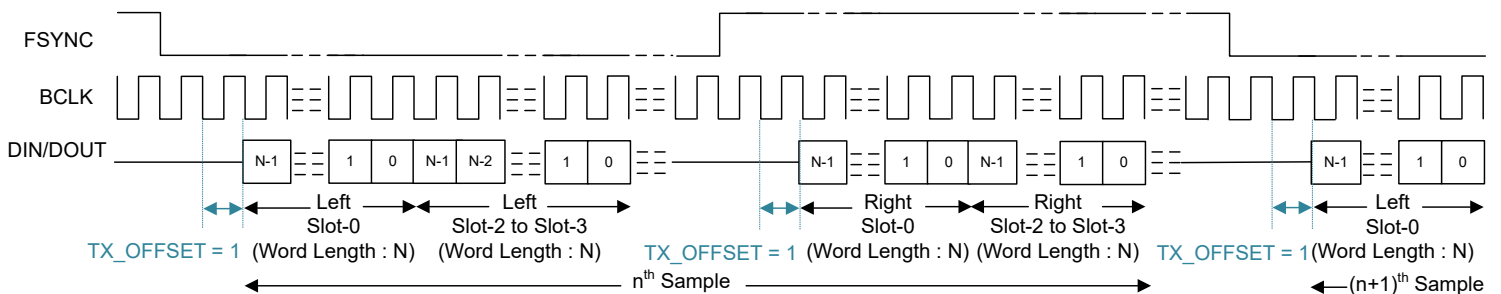
図 6-6. I 2 S Protocol Timing (PASI_TX_OFFSET = 1)
