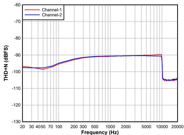
Single-ended headphone output, 16Ω load (-1dBFS input)
