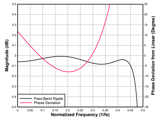
図 6-53. Ultra-Low-Latency interpolation Filter Pass-Band Ripple and Phase Deviation
