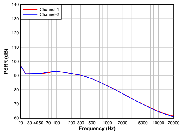
Figure 5-19. DAC PSRR vs Frequency
