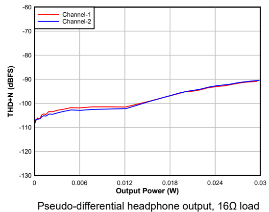
図 5-10. DAC THD+N Level vs output power
