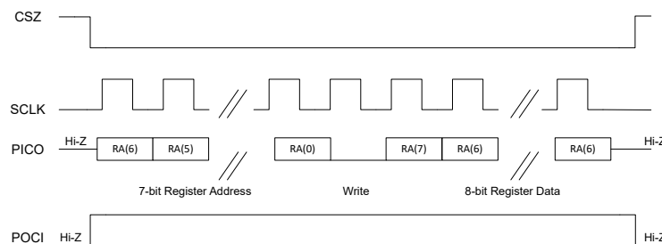
図 6-106. SPI Single-Byte Write Transfer
