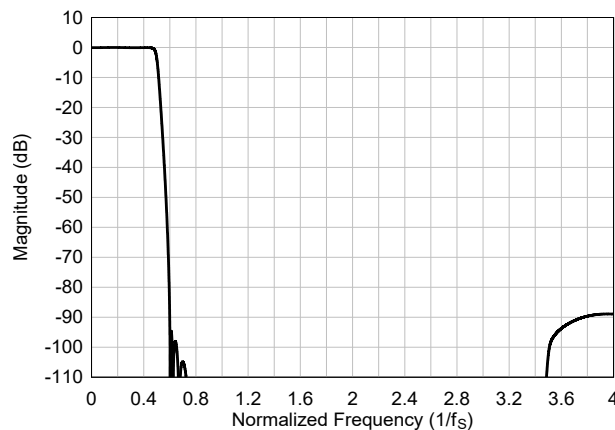
図 6-52. Ultra-Low-Latency interpolation Filter Magnitude Response
