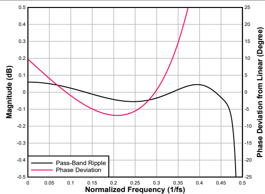
6-99. Ultra Low-latency Decimation Filter Pass-Band Ripple and Phase Deviation
