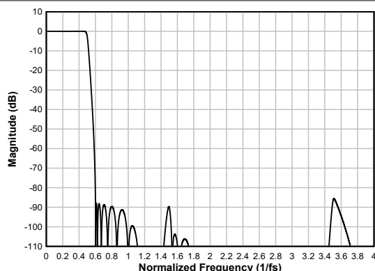
図 6-96. Ultra Low-latency Decimation Filter Magnitude Response
