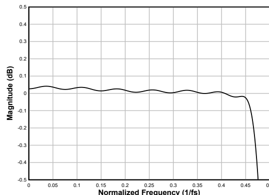
図 6-65. Linear-phase Decimation Filter Pass-Band Ripple
