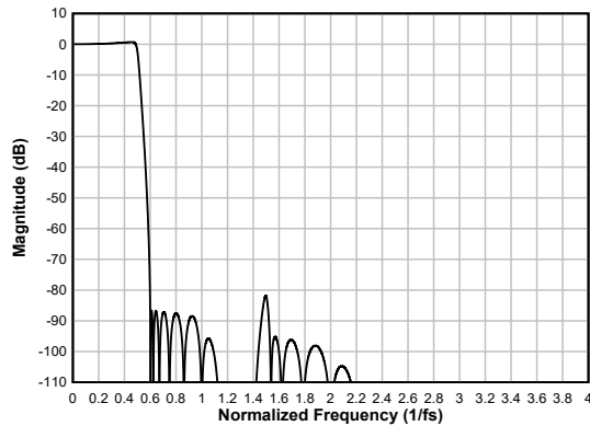
図 6-82. Low-latency Decimation Filter Magnitude Response
