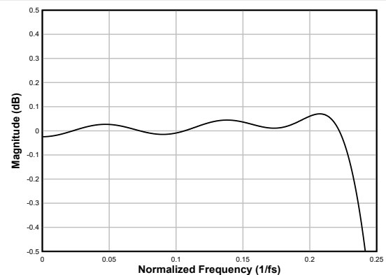
図 6-77. Linear-phase Decimation Filter Pass-Band Ripple
