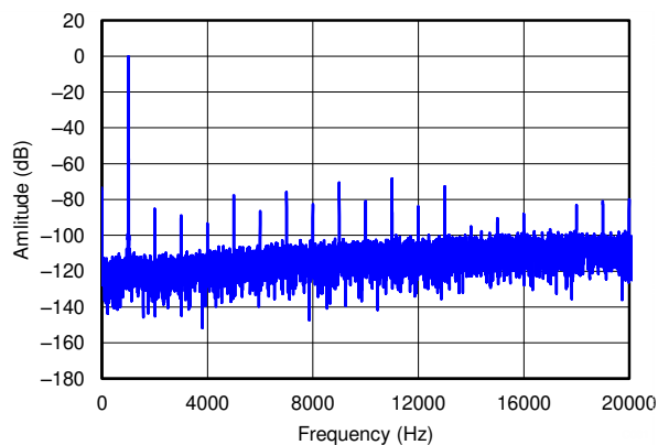
図 5-7. DAC To Speaker Amplitude at 0dBFS vs Frequency
