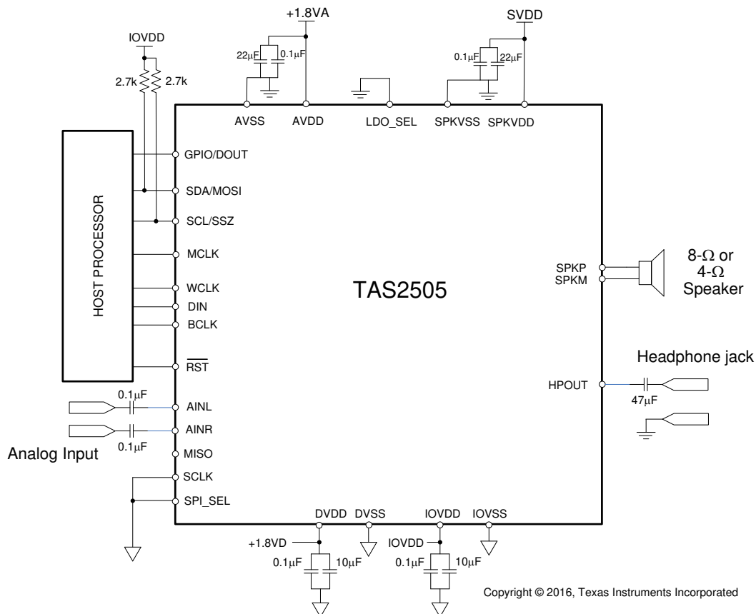
図 9-1. Typical Circuit Configuration
