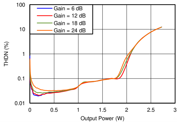
図 5-9. Total Harmonic Distortion + Noise vs 4Ω Speaker Power
