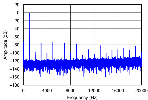
図 5-8. AINL To Speaker FFT Amplitude at 0dBFS vs Frequency
