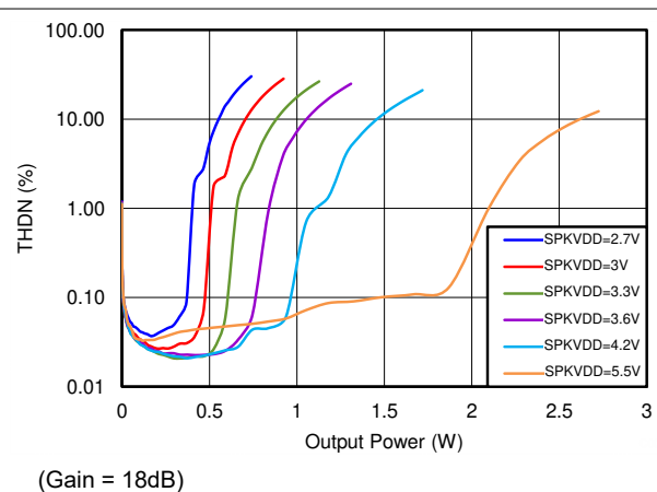
図 9-3. Total Harmonic Distortion + Noise vs 4Ω Speaker Power
