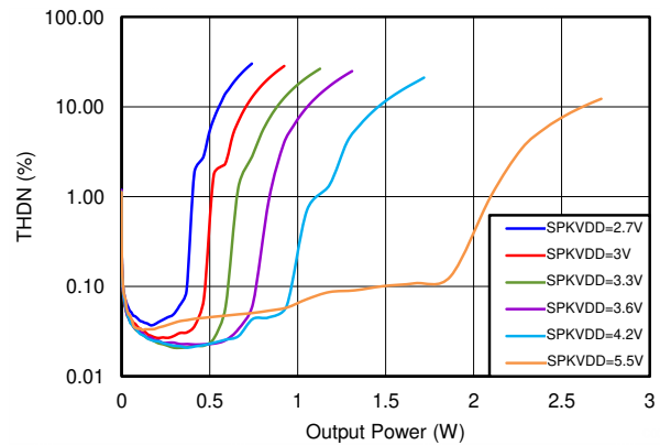
図 5-10. Total Harmonic Distortion + Noise + NOISE vs 4Ω Speaker Power
