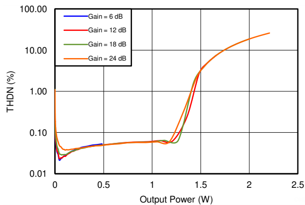
図 5-11. Total Harmonic Distortion + Noise + NOISE vs 8Ω Speaker Power
