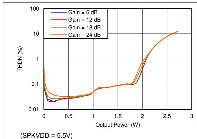
図 9-2. Total Harmonic Distortion + Noise vs 4Ω Speaker Power
