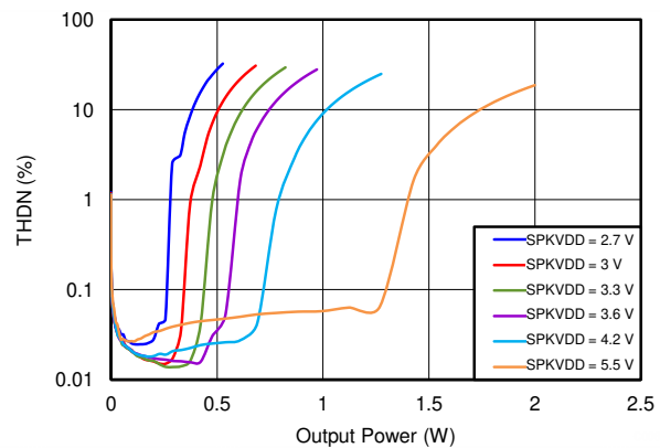
図 5-12. Total Harmonic Distortion + Noise + NOISE vs 8Ω Speaker Power
