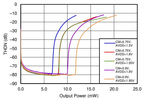
5-17. Total Harmonic Distortion + Noise vs HP Power
